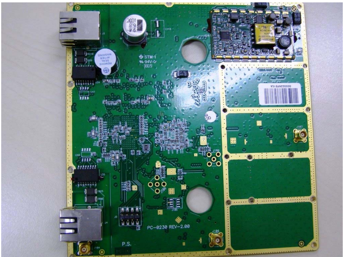
Internal picture close-up
