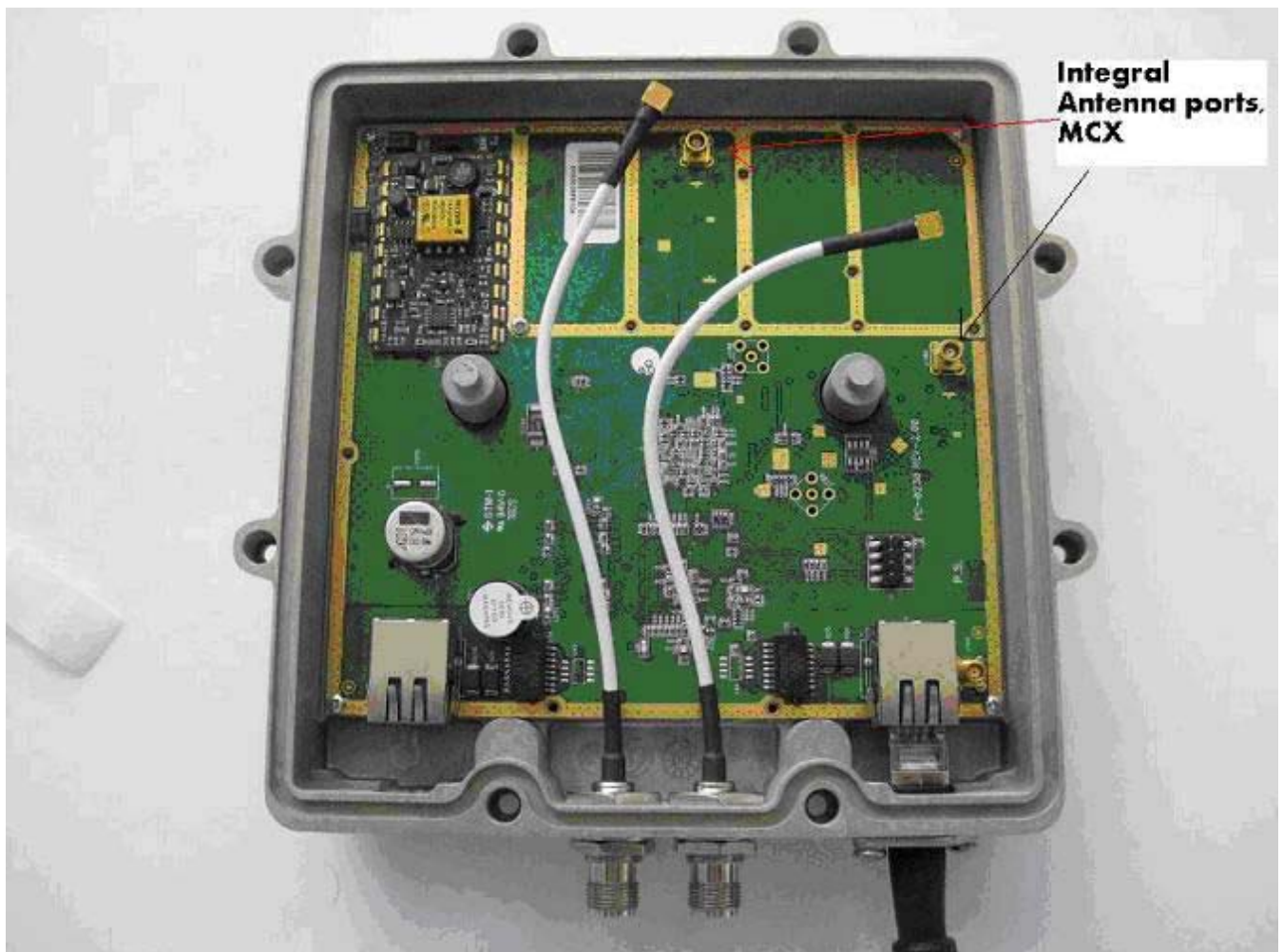
Internal picture with integrated antenna ports (MCX connectors)
