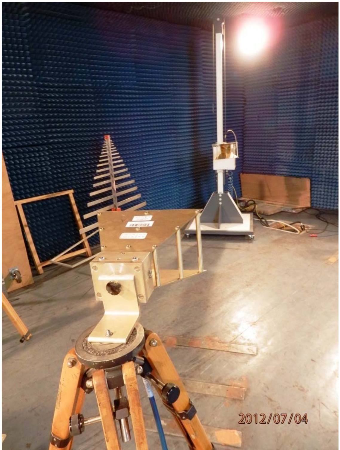
Photograph for Substitution of ERP Test Setup
