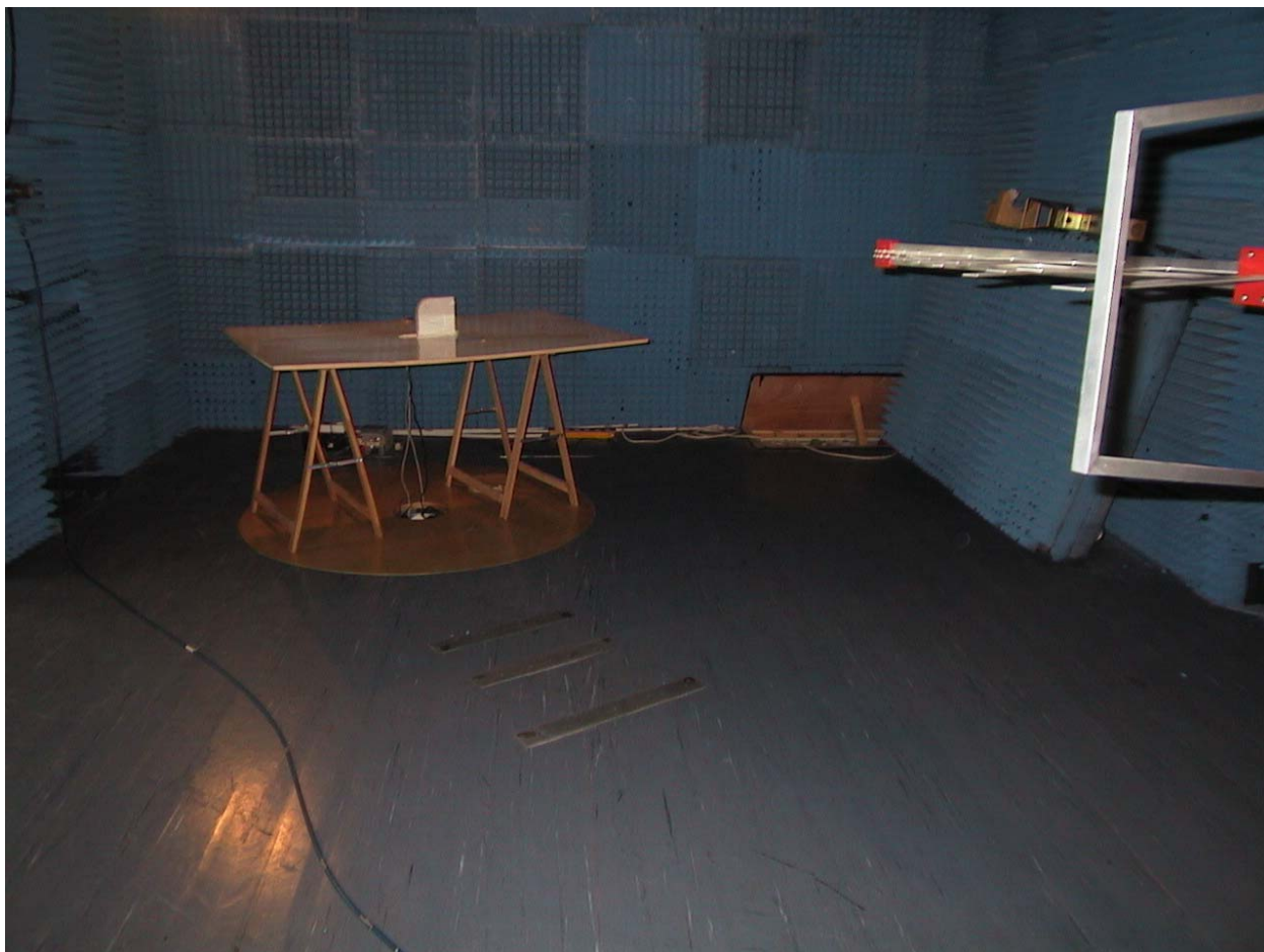
Radiated emission 30MHz – 1GHz Setup
