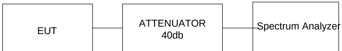
Figure 6e Test Setup for Conducted emission
