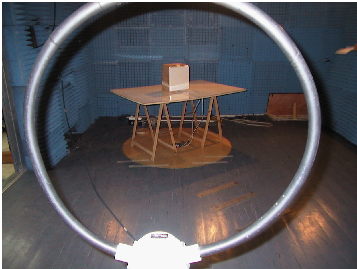
Radiated emission up to 30MHz Setup
