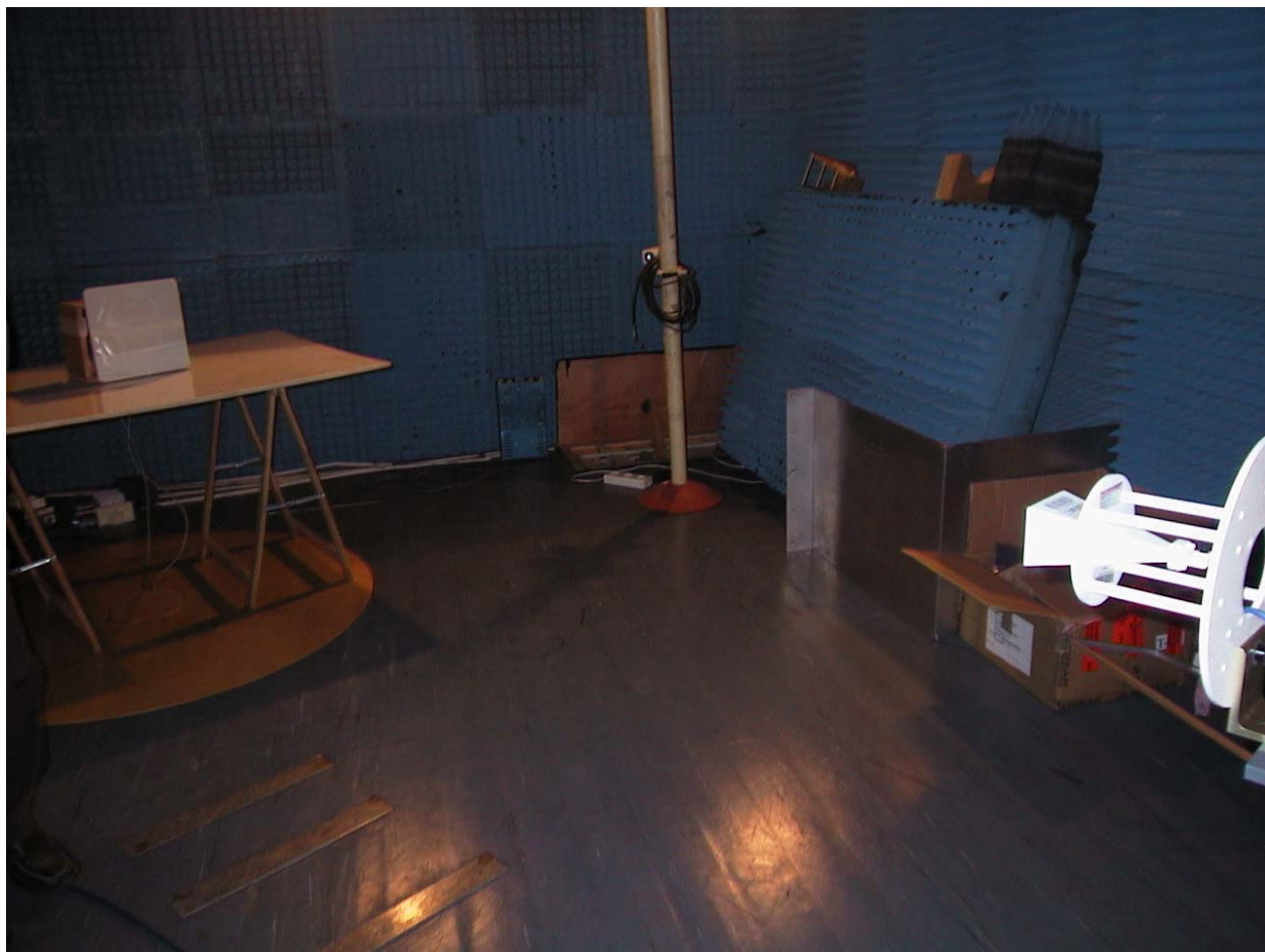
Radiated emission 18GHz – 40GHz Setup
