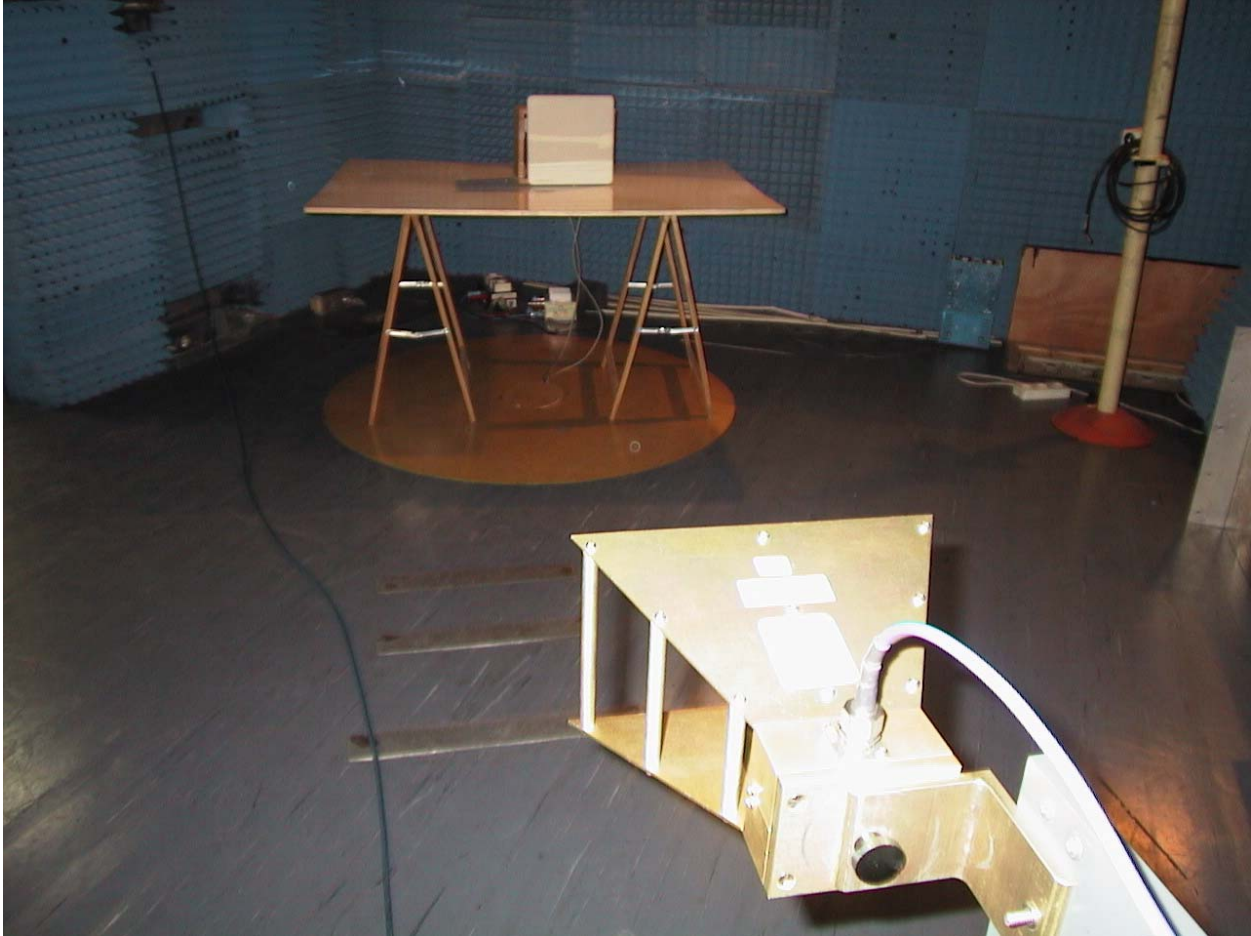
Radiated emission 1GHz – 18GHz Setup
