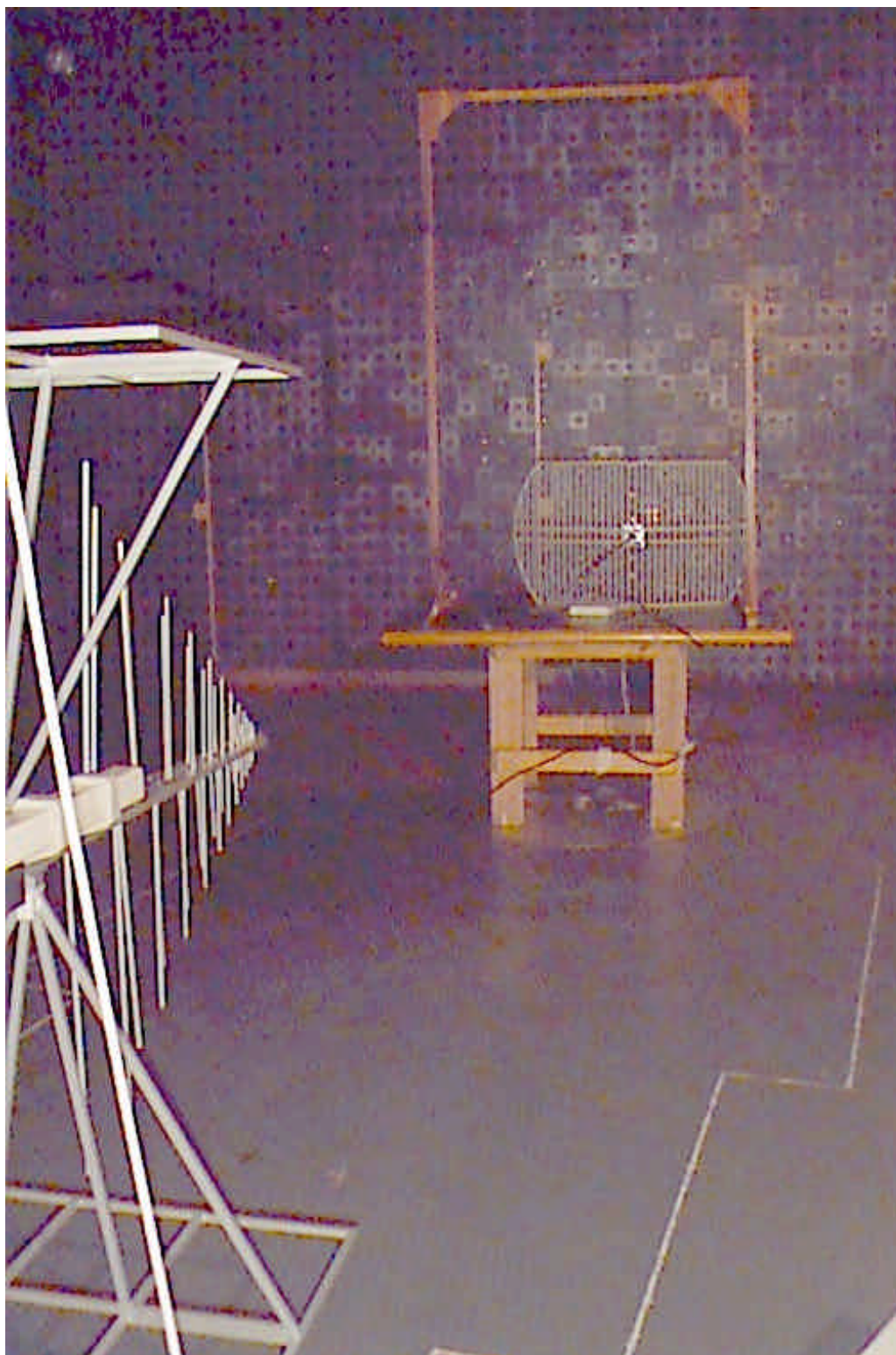
Photograph No.13 Radiated emissions measurement setup view with 24 dBi antenna
