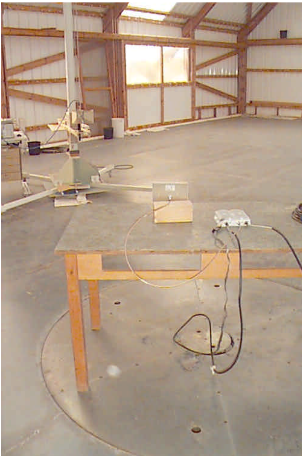
Photograph No.3 Radiated emissions measurement setup general view with 13.5 dBi antenna
