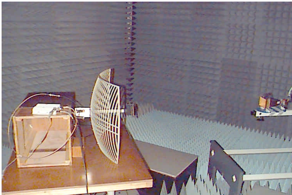
Photograph No.15 Radiated emissions measurement setup view with 24 dBi antenna in 18 – 24 GHz
