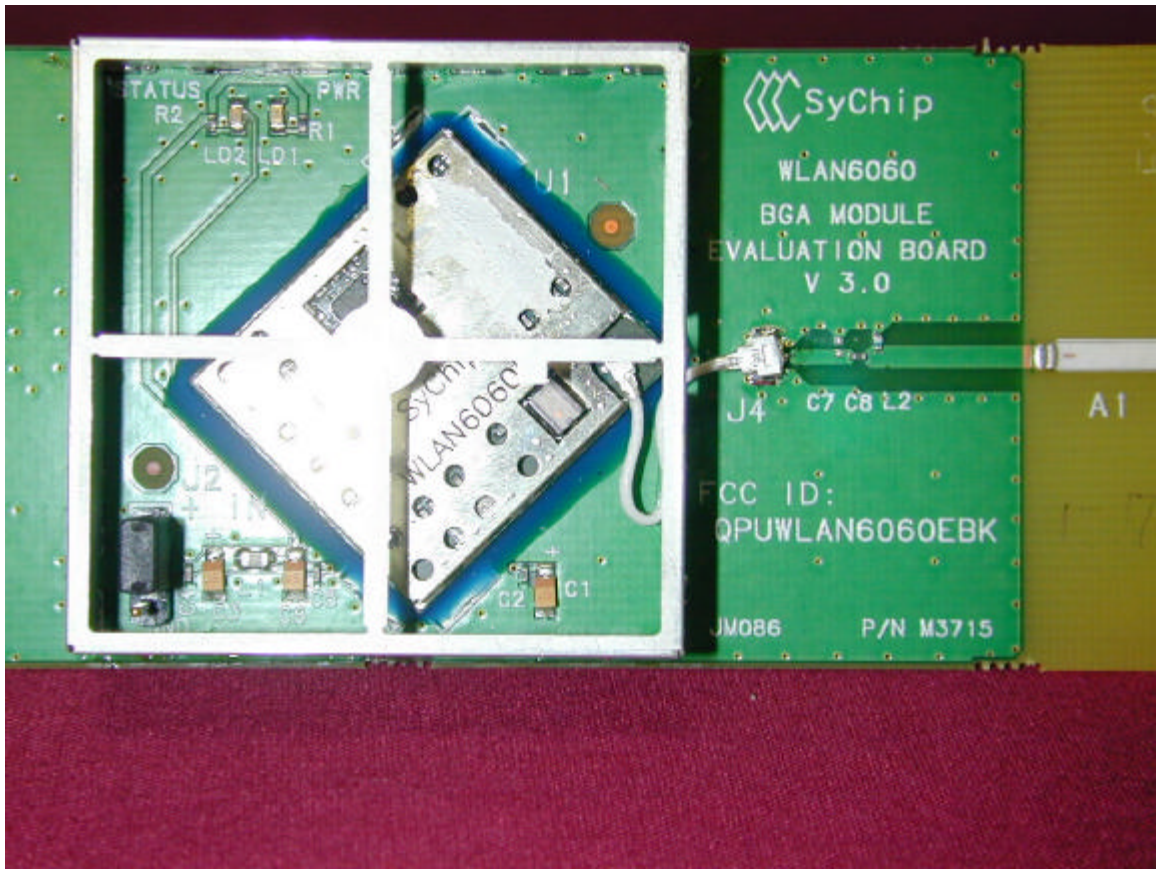
PCB Top Closeup with shield removed
