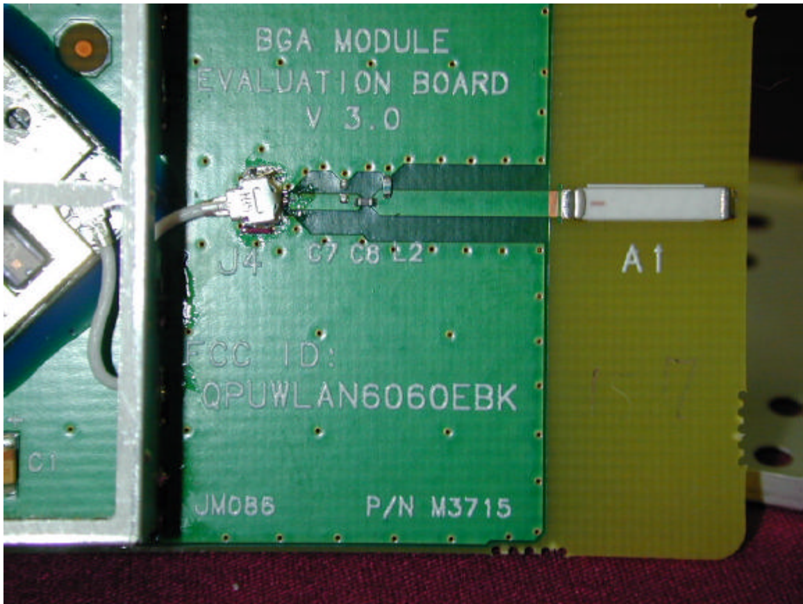
PCB Closeup of Antenna Connection
