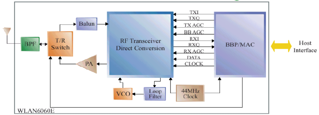
Figure 1. WLAN6060BB(EB) Block Diagram
