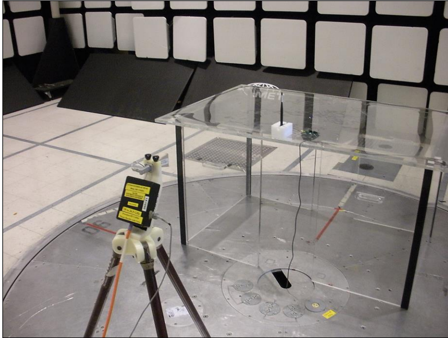
Photograph 3. Radiated Spurious Emissions, Test Setup, 18 GHz – 26.5 GHz
