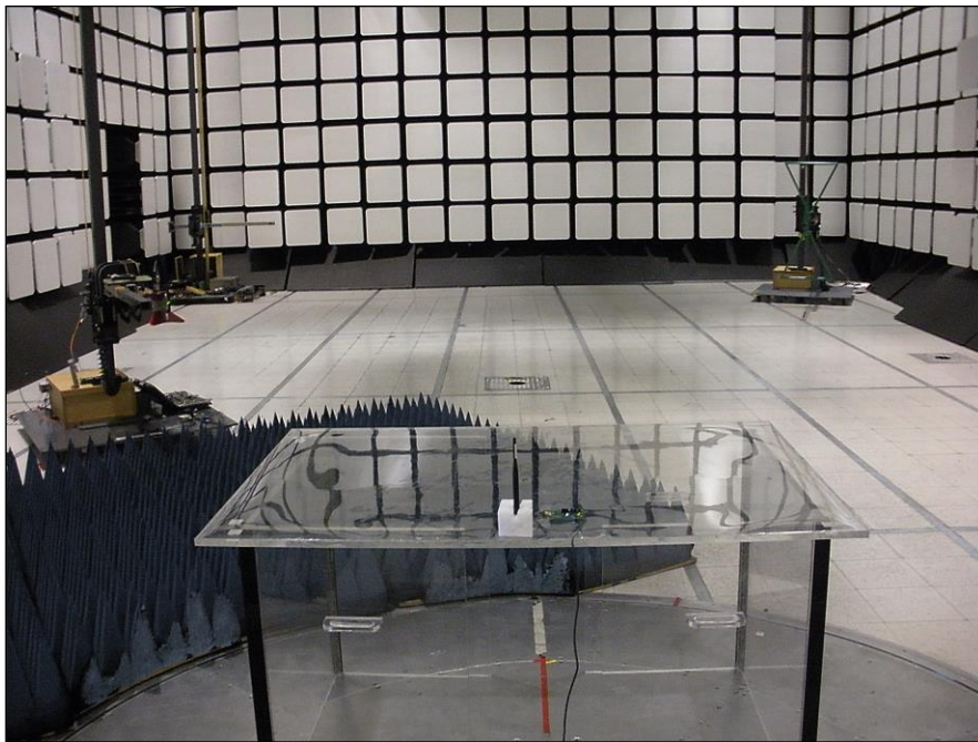
Photograph 4. Radiated Spurious Emissions, Test Setup, Rear
