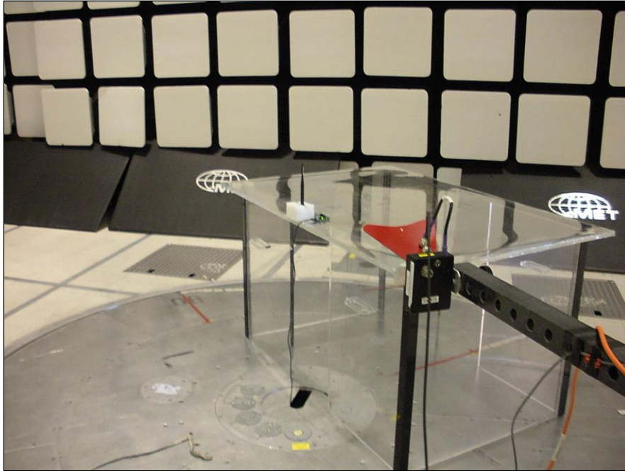
Photograph 5. Radiated Restricted Band, Test Setup
