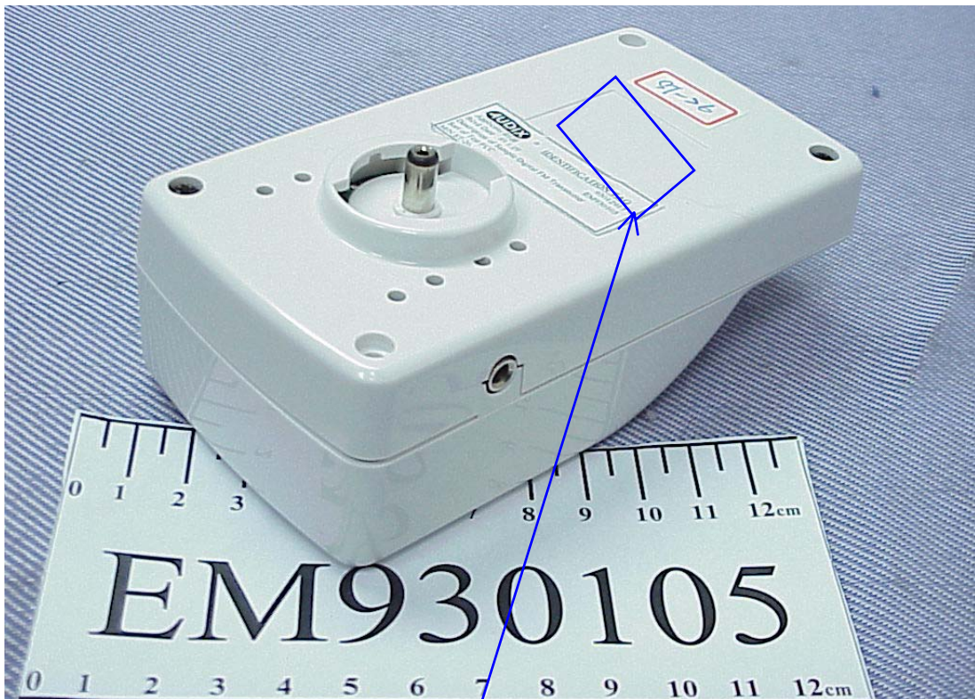
FCC Label Placement Location
