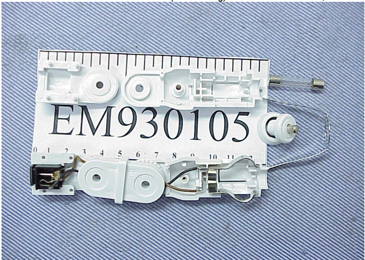
Photos 4 (Power Plug) Remove Case Cover, Internal View
