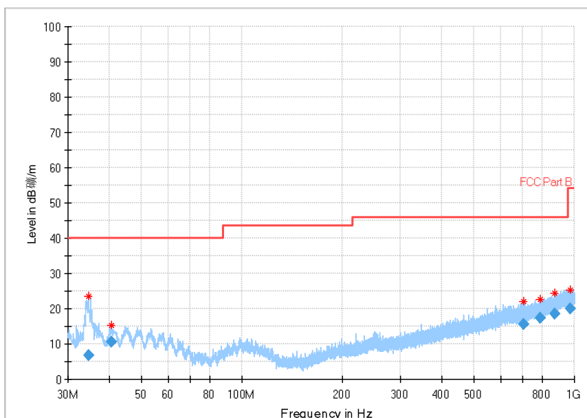
Fig.109 Radiated Spurious Emission (802.11 n-20MHz,Ch11,30MHz~1GHz)
