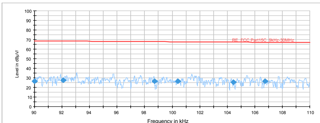
FCC RE 90K-110kHz QP
