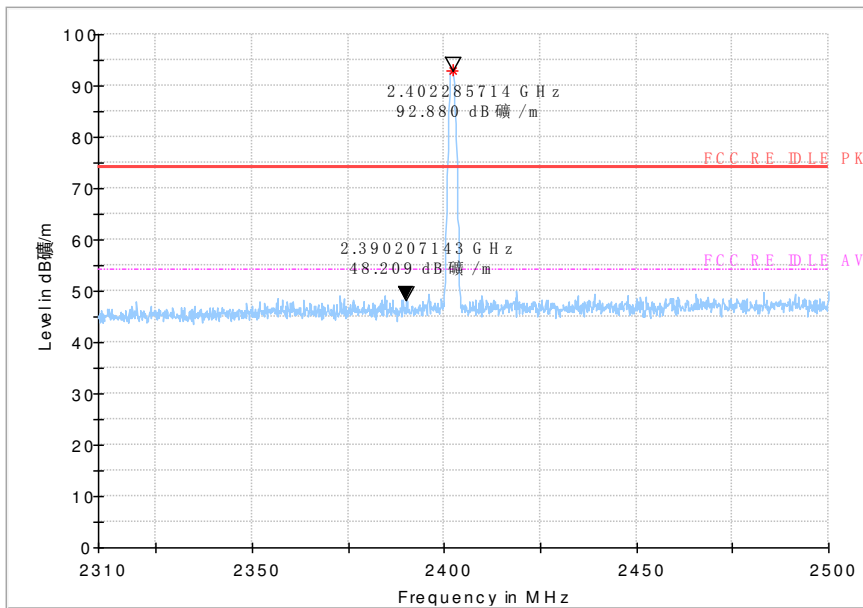
Peak detector Bandedge:ch0
