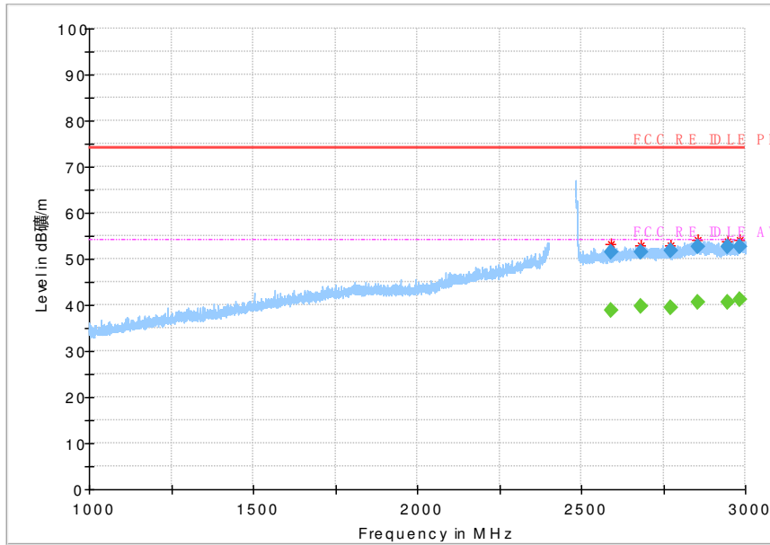
Fig.105 Radiated Spurious Emission (802.11g,Ch11,1GHz~3GHz)
