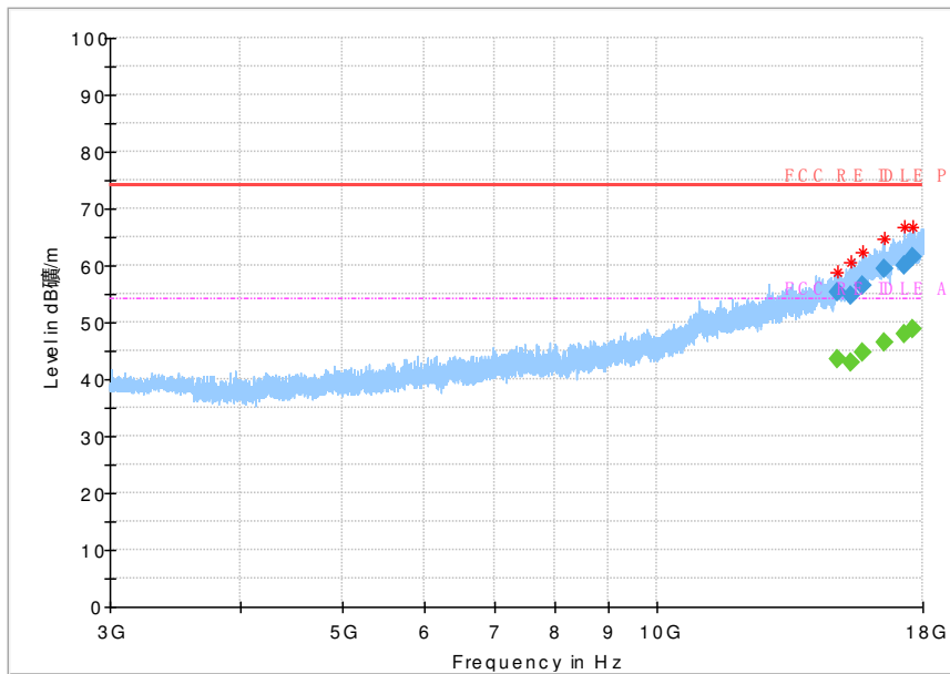
Fig.106 Radiated Spurious Emission (802.11g,Ch11,3GHz~18GHz)
