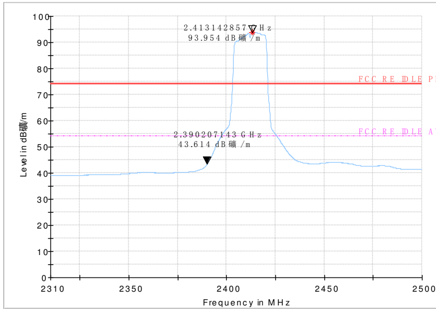
Fig.102 Radiated emission (Power): 802.11g, low channel
