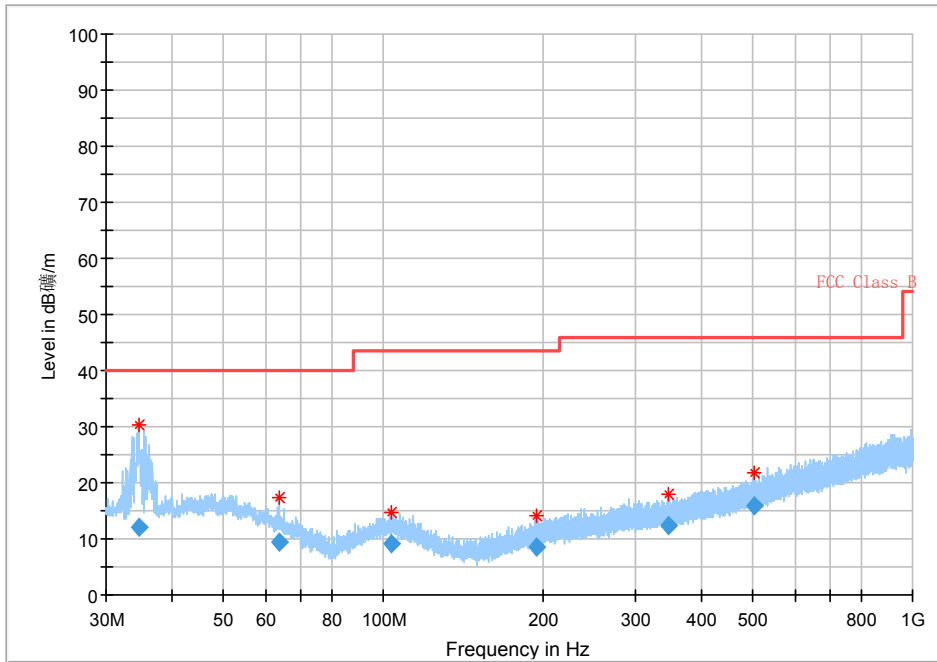
Fig. 36 Radiated Spurious Emission (802.11n-HT40, Ch159, 30 MHz-1 GHz)
