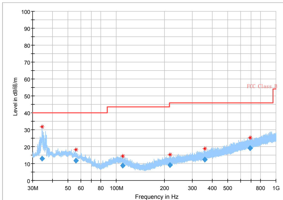
Fig. 26 Radiated Spurious Emission (802.11a, Ch165, 30 MHz-1 GHz)
