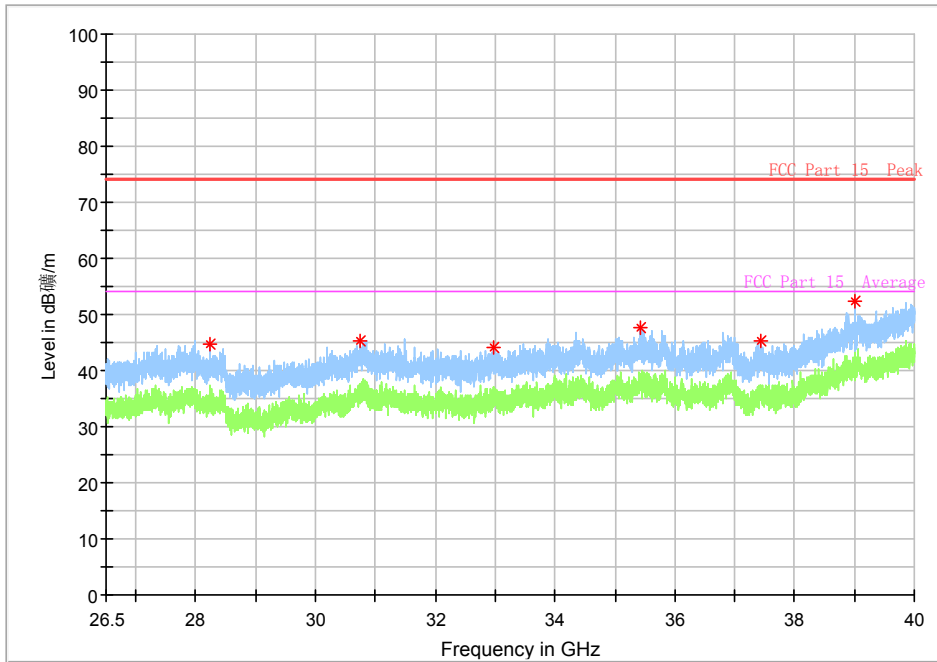
Fig. 40 Radiated emission: 802.11n, (802.11n-HT40, Ch159, 26.5 GHz - 40 GHz)
