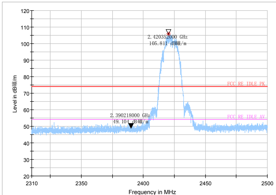
Peak detector
