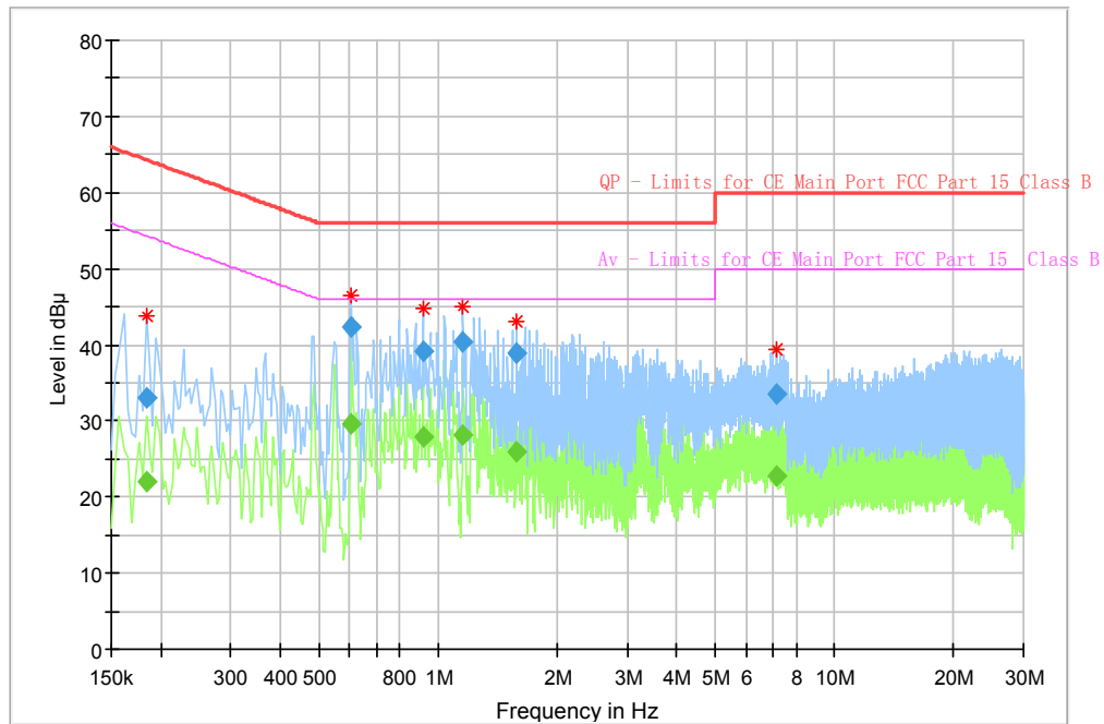
Fig 77. AC Powerline Conducted Emission
