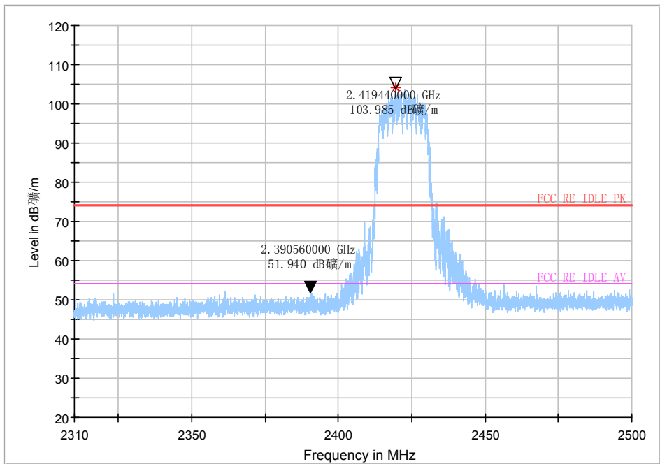
Peak detector
