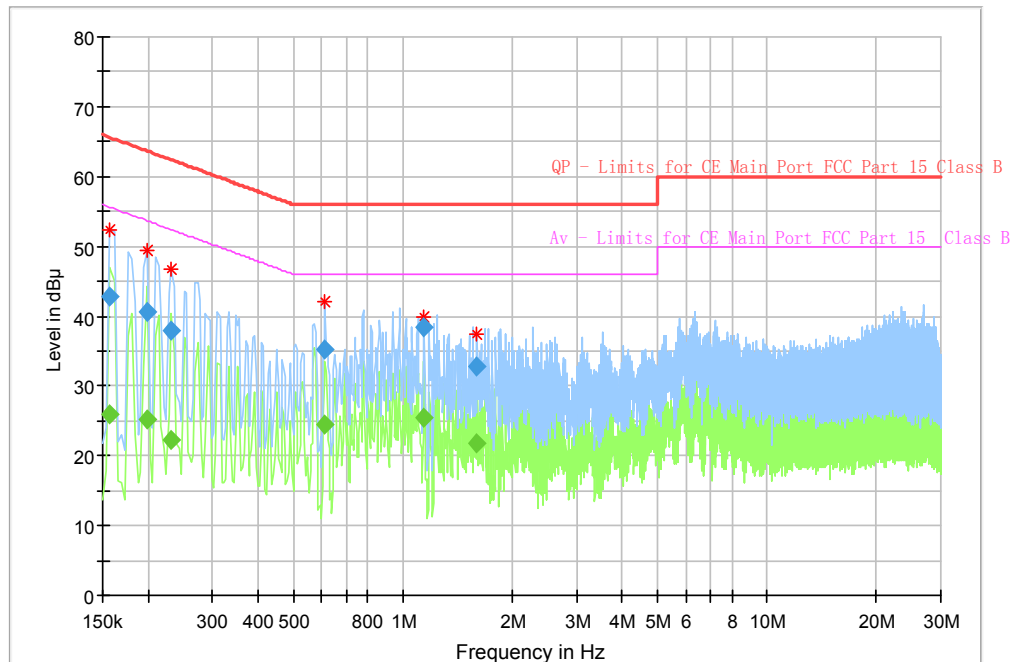
Fig.26 AC Powerline Conducted Emission
