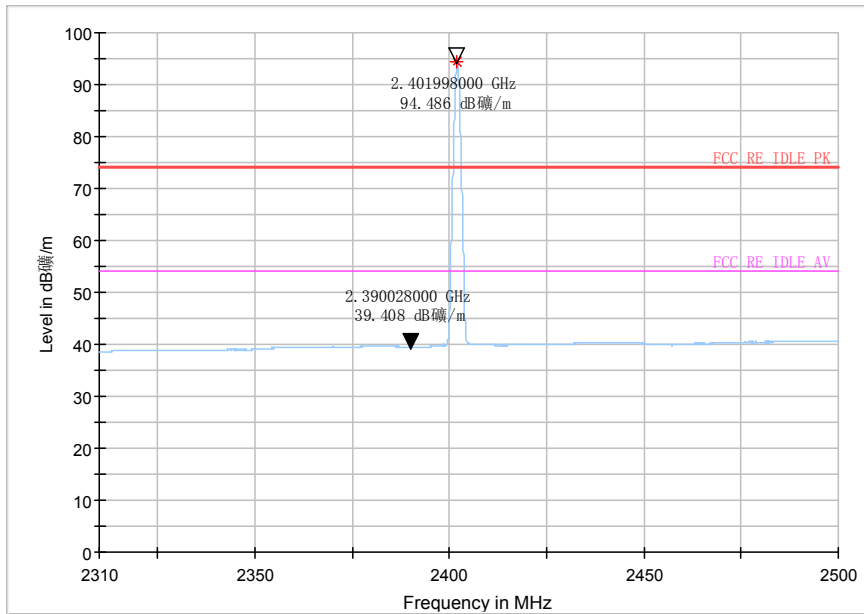
Fig.21 Bandedge:ch0
