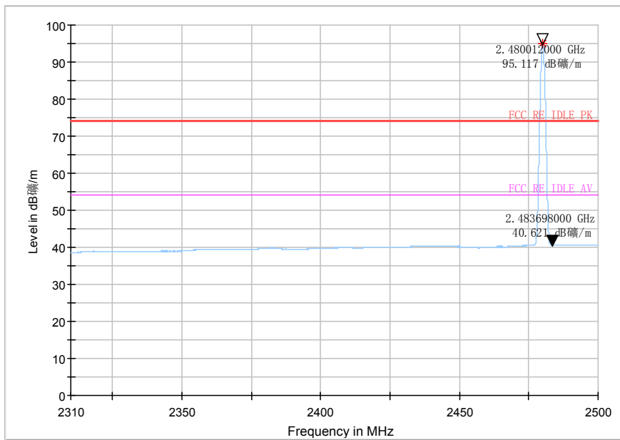
Fig.25 Bandedge:ch39
