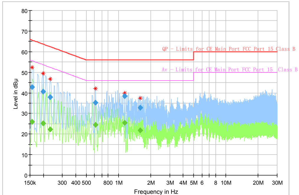
Fig.82 AC Powerline Conducted Emission
