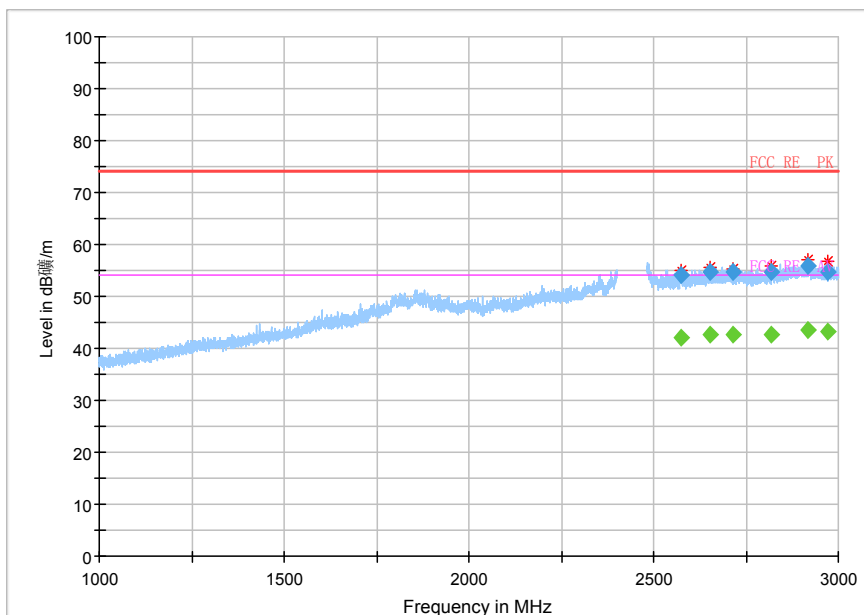
Fig.37 Radiated emission: \pi/4 DQPSK, Ch78, 1GHz~3GHz
