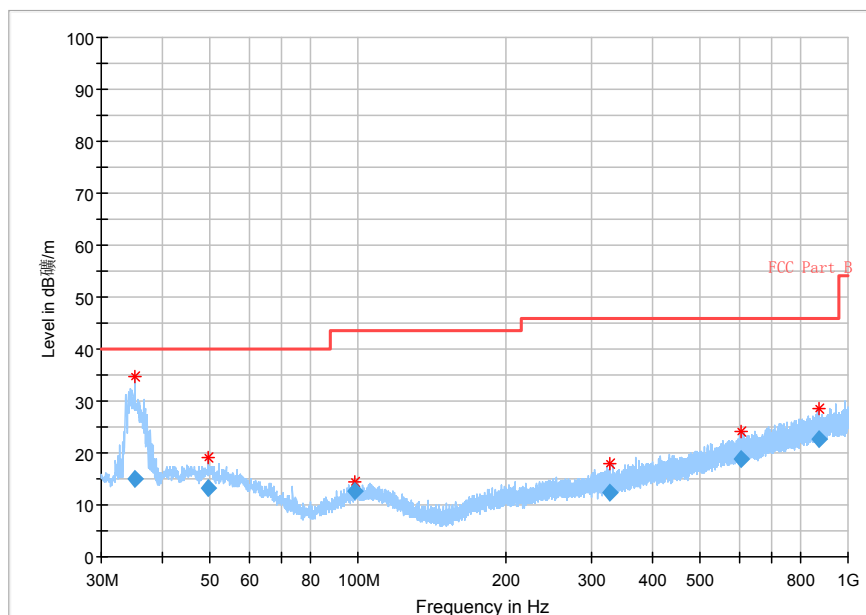
Fig.31 Radiated emission: GFSK, Ch78, 30MHz~1GHz
