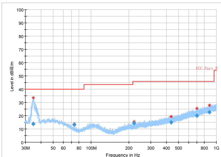
Fig.36 Radiated emission: \pi/4 DQPSK, Ch78, 30MHz~1GHz
