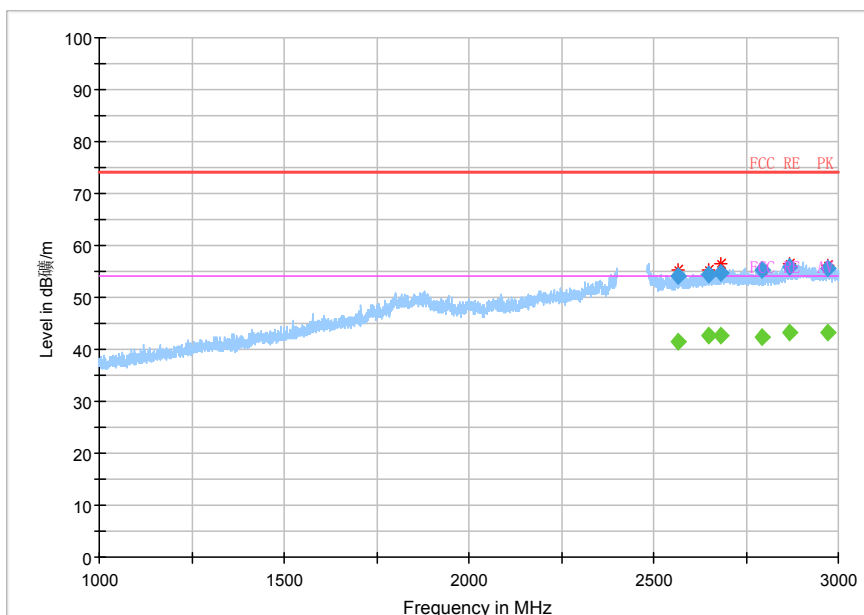
Fig.42 Radiated emission: 8DPSK, Ch78, 1GHz~3GHz
