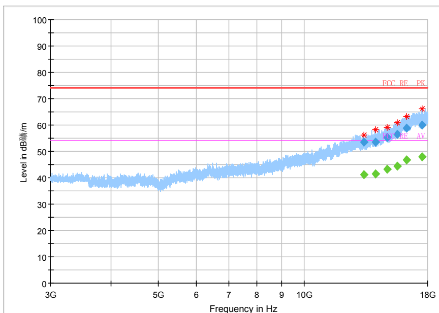
Fig.43 Radiated emission: 8DPSK, Ch78, 3GHz~18GHz
