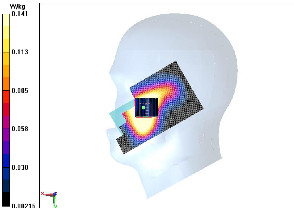
Fig.5 GSM1900 Right Cheek Middle
