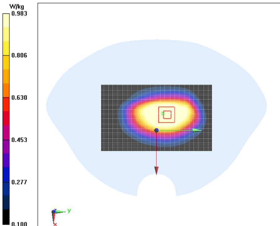
Fig.2 GSM850 Ground Mode Middle 10mm
