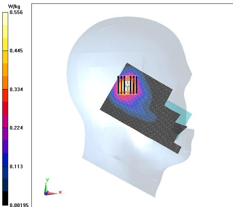
Fig.9 WiFi 802.11b Left Cheek Middle
