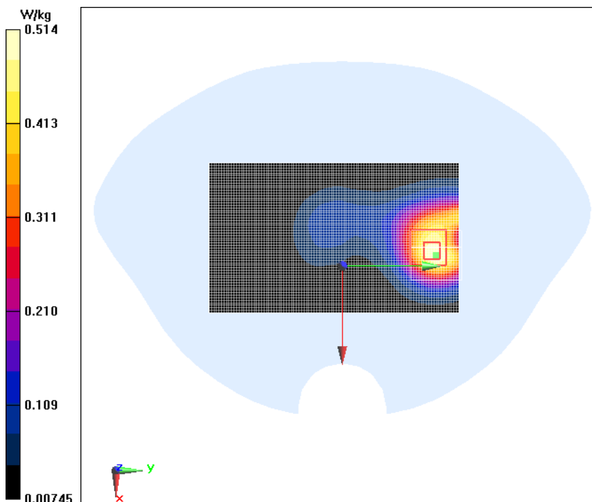
Fig.6 GSM1900 Ground Mode High 10mm
