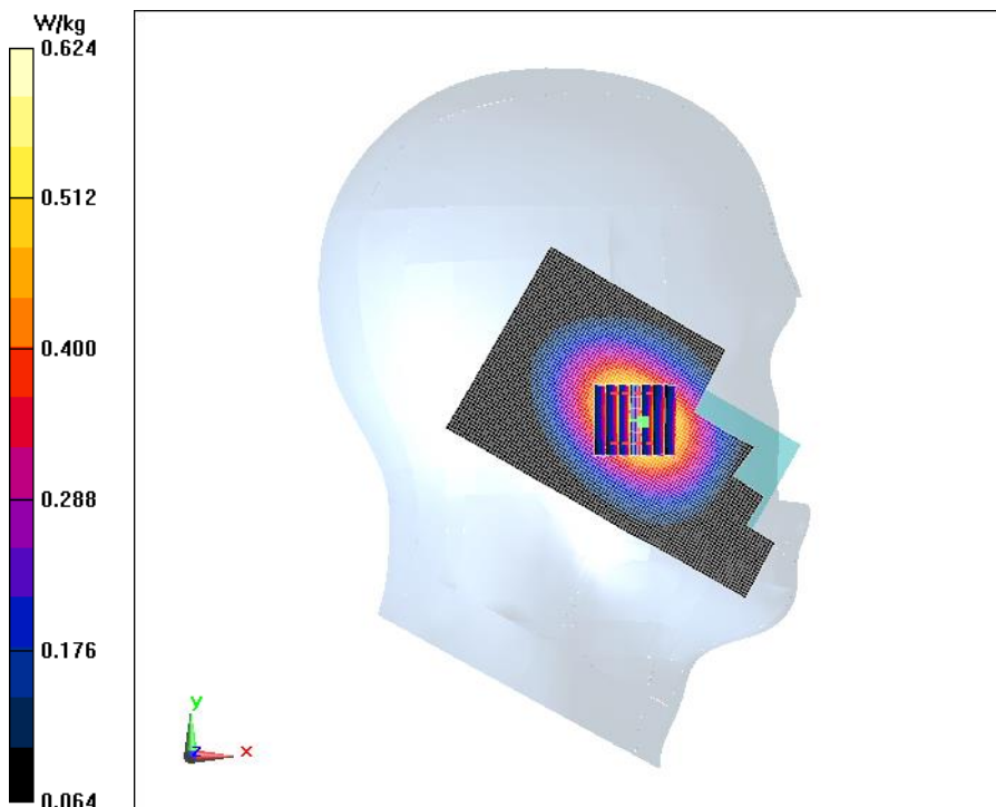
Fig.1 GSM850 Left Cheek Low
