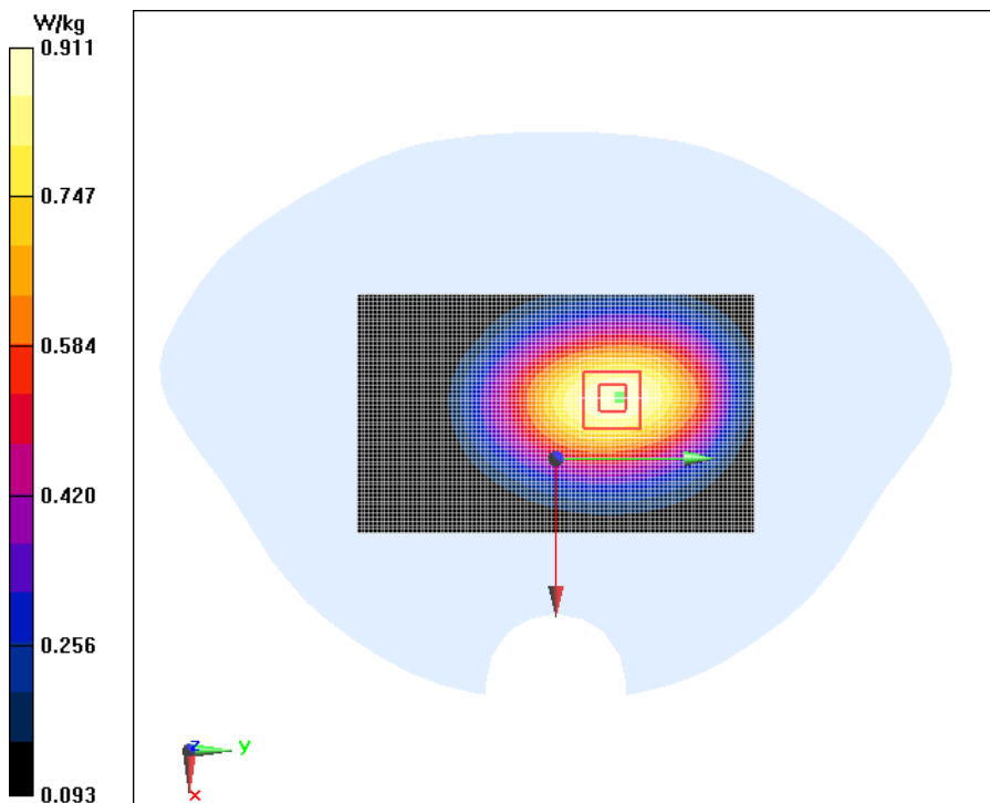
Fig.3 GSM850 Phantom Mode Low 10mm
