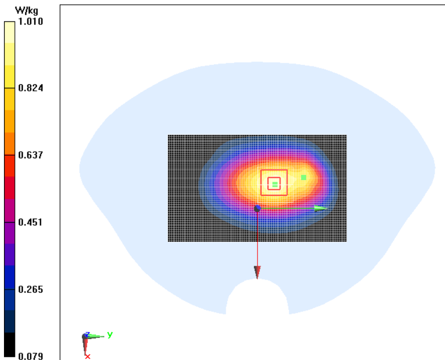
Fig.4 GSM850 Ground Mode Middle 10mm Repeated
