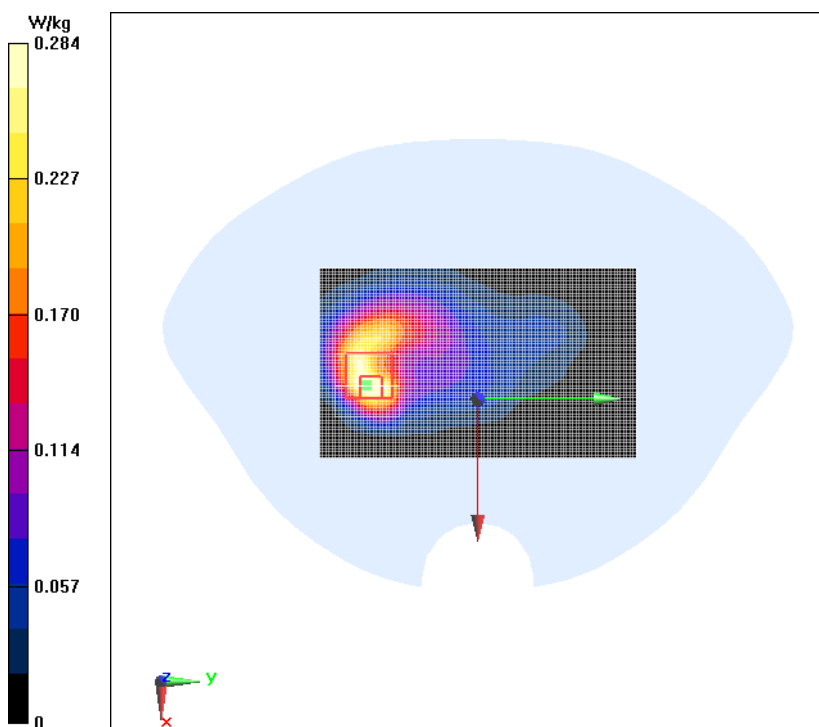
Fig.10 WiFi 802.11b Ground Mode High
