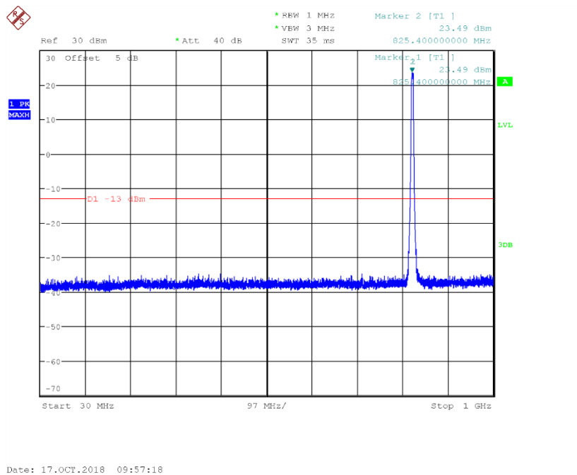
Fig.83 Channel 4132: 30MHz~1GHz
