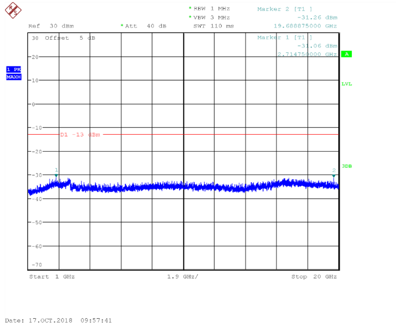
Fig.84 Channel 4132: 1GHz~20GHz
