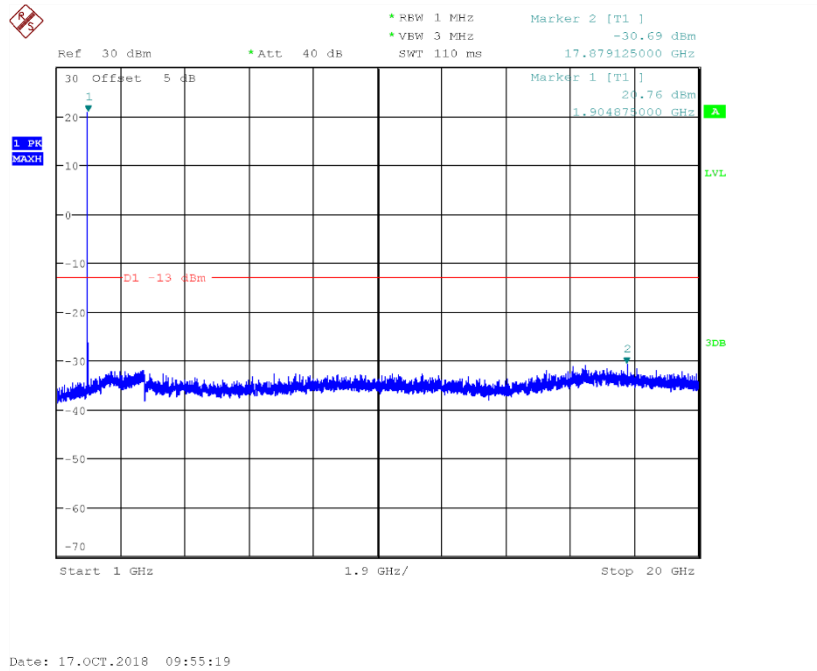
Fig.82 Channel 9538: 1GHz~20GHz
