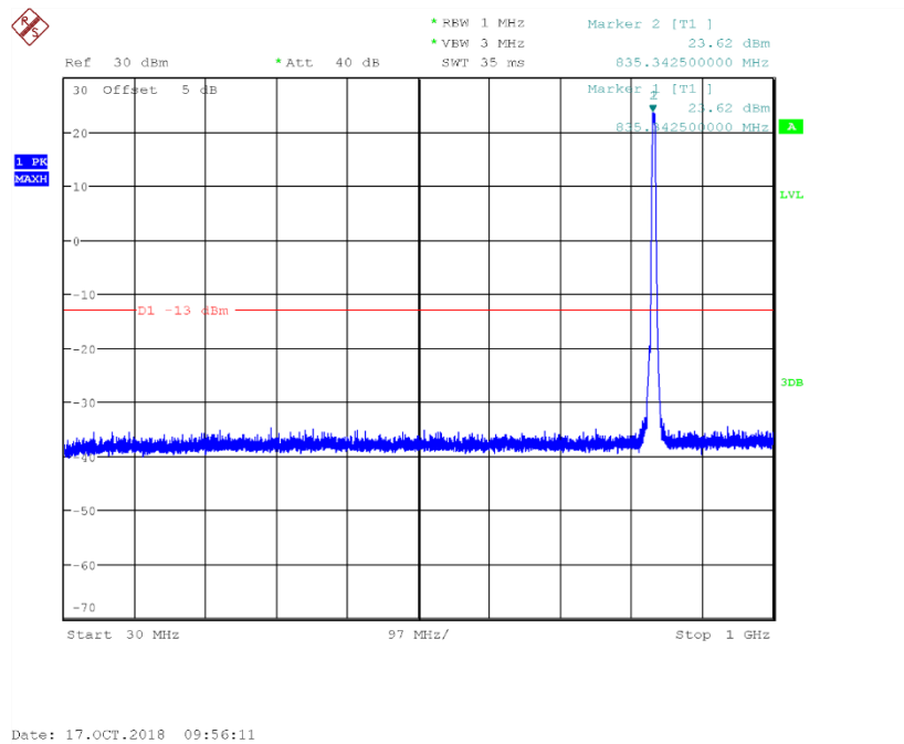
Fig.85 Channel 4183: 30MHz~1GHz
