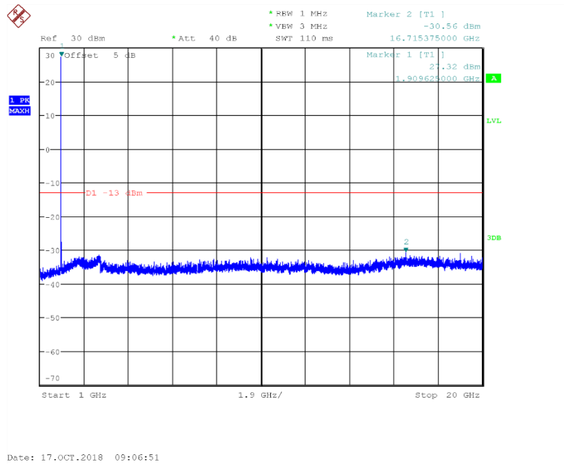
Fig.76 Channel 810: 1GHz~20GHz
