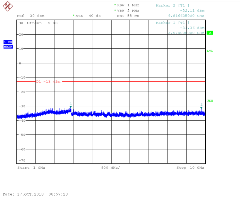
Fig.68 Channel 189: 1GHz~10GHz
