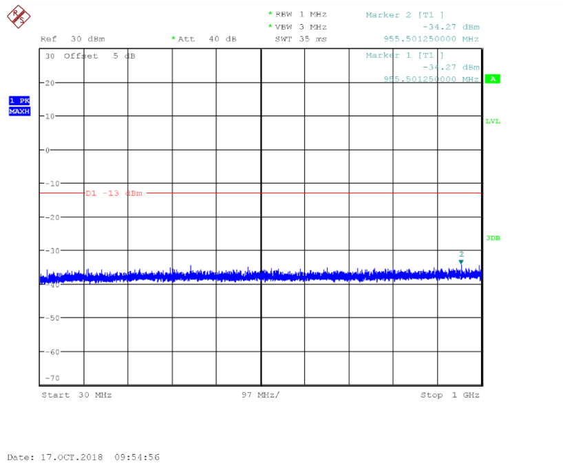
Fig.81 Channel 9538: 30MHz~1GHz
