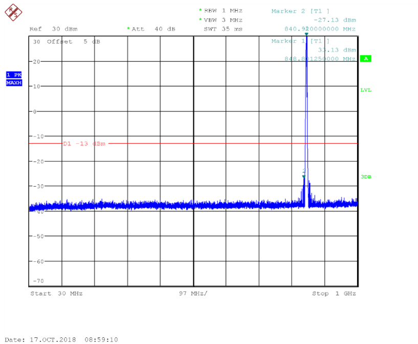
Fig.69 Channel 251: 30MHz~1GHz
