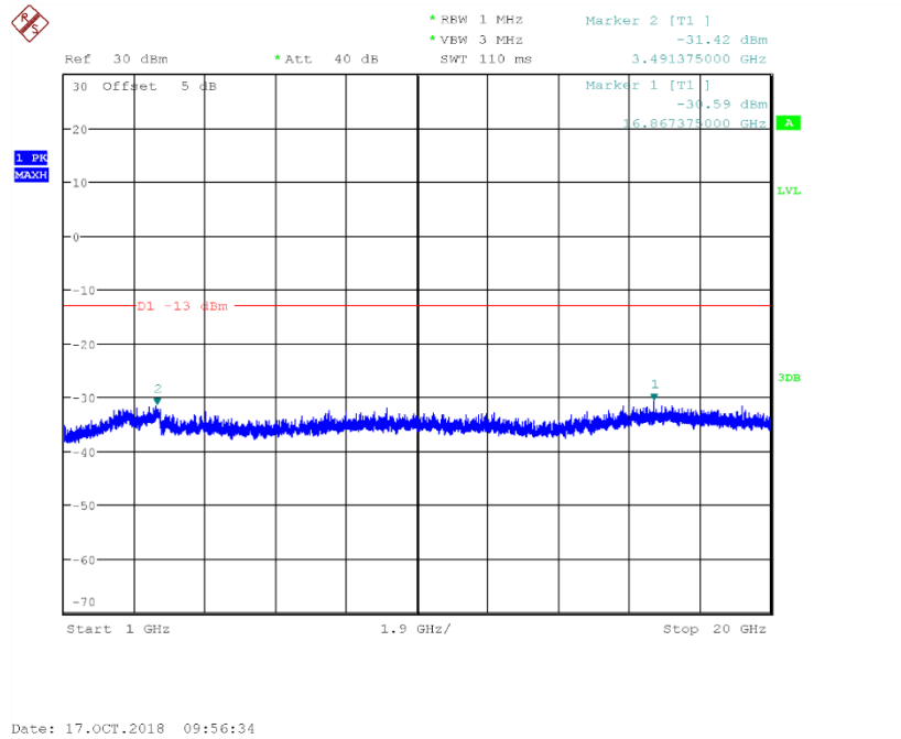
Fig.86 Channel 4183: 1GHz~20GHz
