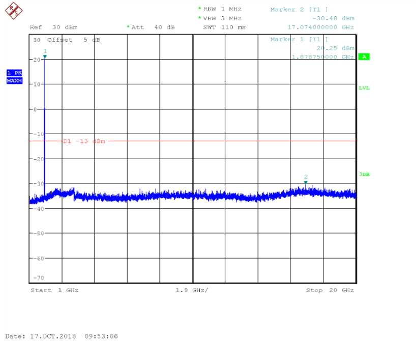
Fig.80 Channel 9400: 1GHz~20GHz
