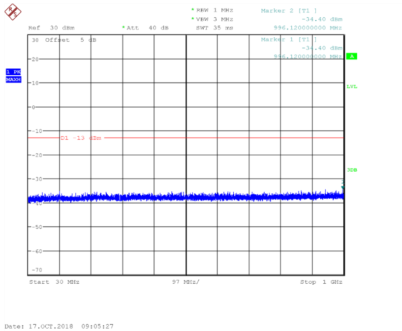
Fig.71 Channel 512: 30MHz~1GHz
