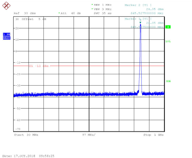
Fig.87 Channel 4233: 30MHz~1GHz
