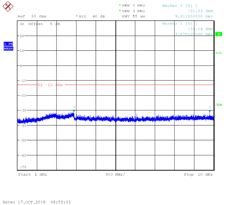
Fig.70 Channel 251: 1GHz~10GHz
