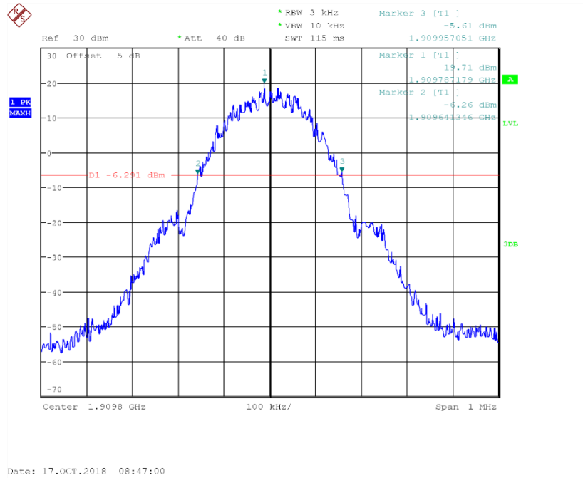
Fig.39 Channel 810- Emission Bandwidth (-26dBc BW)
