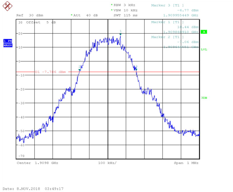
Fig.36 Channel 810- Emission Bandwidth (-26dBc BW)
