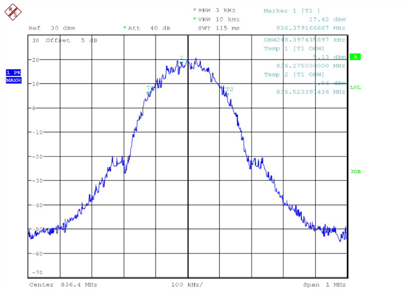
Fig.6 Channel 251-Occupied Bandwidth (99%)
