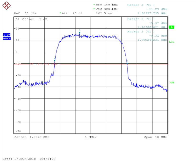
Fig.45 Channel 9538- Emission Bandwidth (-26dBc BW)
