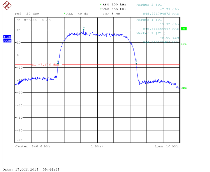
Fig.48 Channel 4233- Emission Bandwidth (-26dBc BW)
