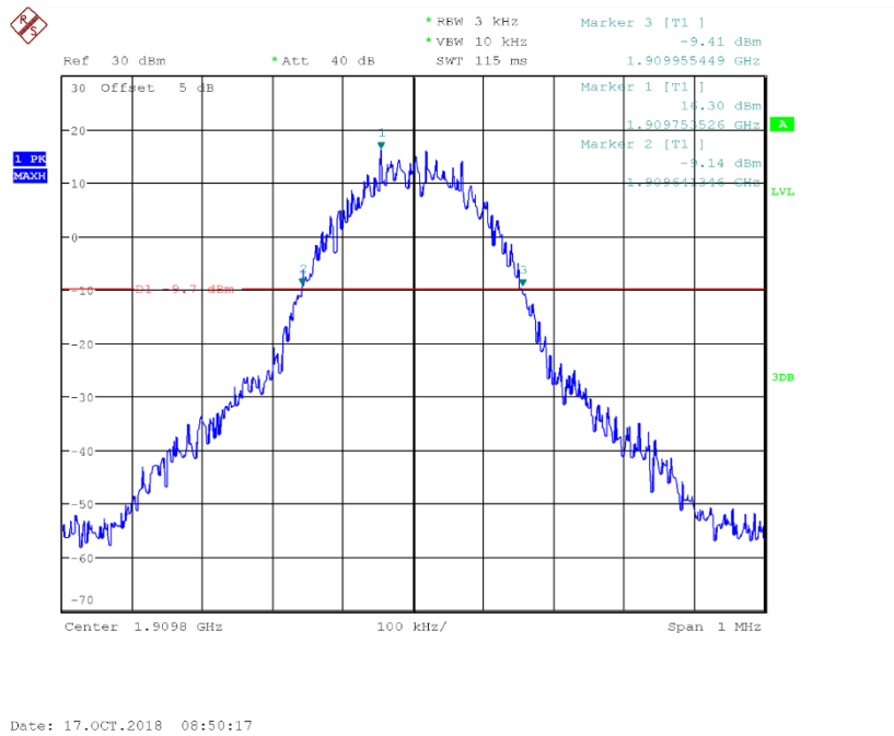
Fig.42 Channel 810- Emission Bandwidth (-26dBc BW)
