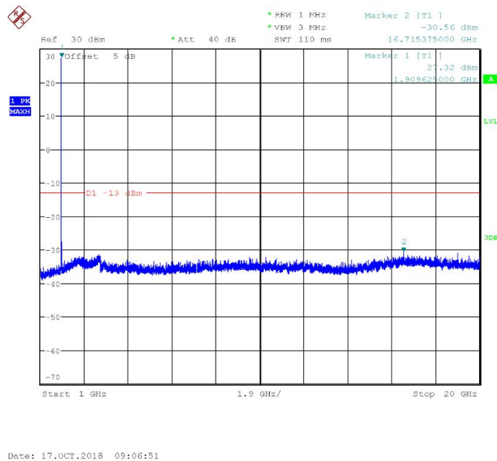
Fig.76 Channel 810: 1GHz~20GHz
