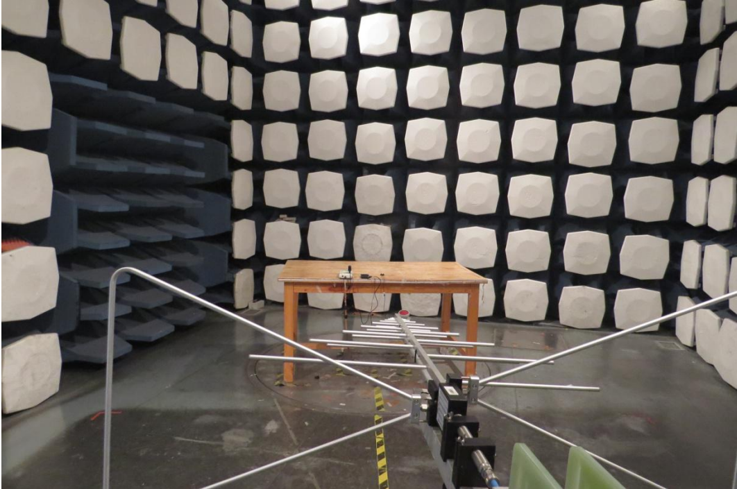
Below 1GHz
