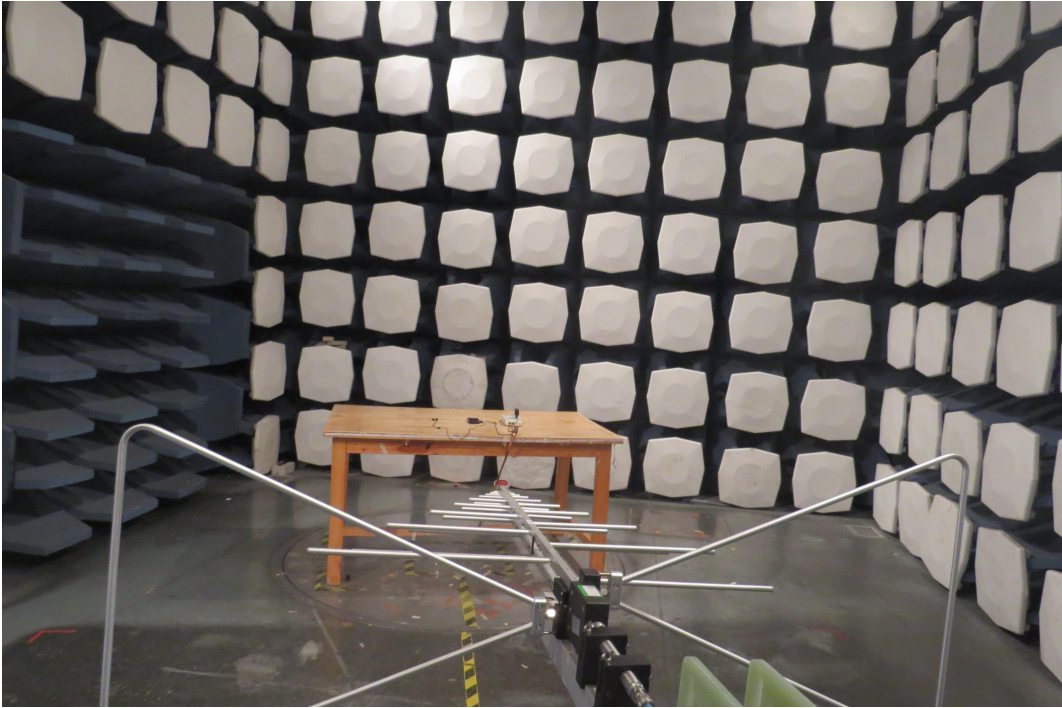
30MHz-1GHz
