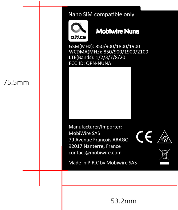
The effect for incoming material 来料示意图
