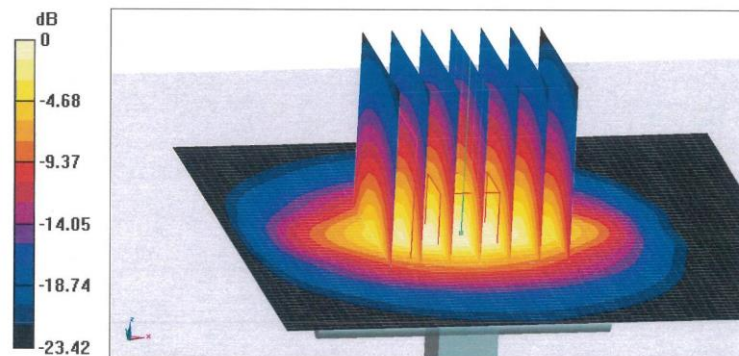
0 dB = 24.5 W/kg = 13.89 dBW/kg
