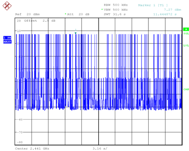
Fig.65 Time of occupancy (Dwell Time): Ch39, Packet 2-DH5
