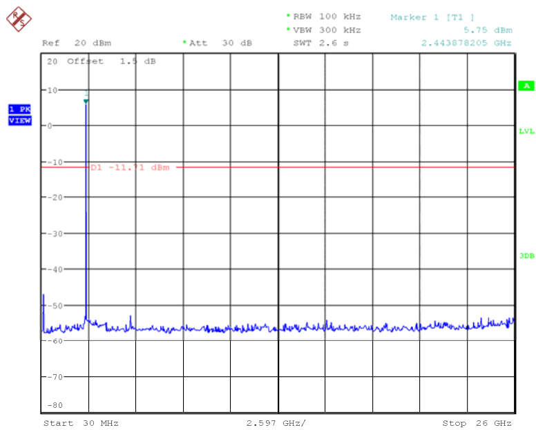
Fig 37. Conducted Spurious Emission (802.11b, Ch11)
