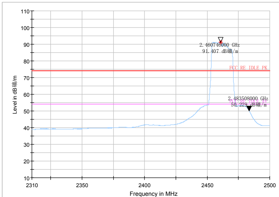
Fig 63. Bandedge: 802.11g, high channel
