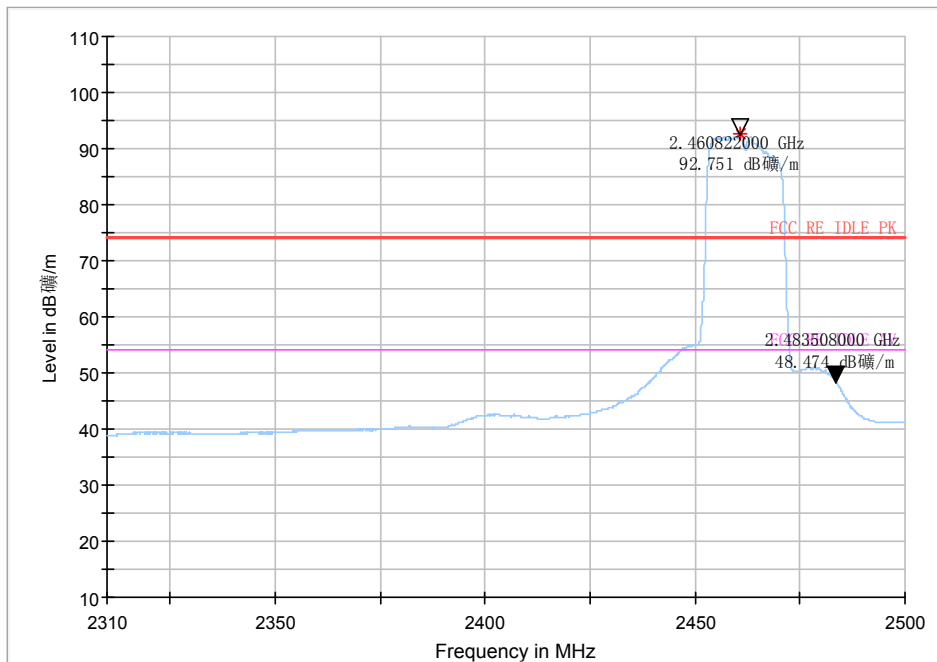
Fig 68. Bandedge: 802.11 n-20MHz, high channel
