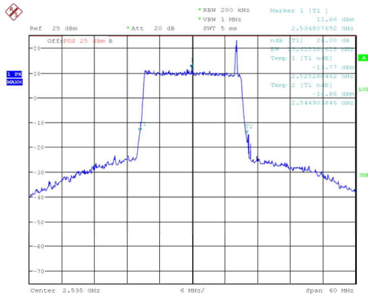
Fig.51 LTE band 7, 20MHz Bandwidth, QPSK (-26dBc BW)
