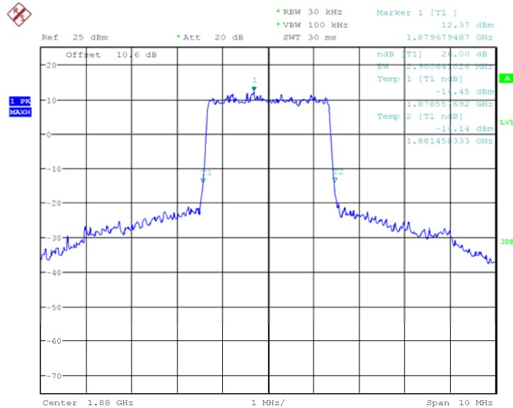
Fig.35 LTE band 2, 3MHz Bandwidth, QPSK (-26dBc BW)
