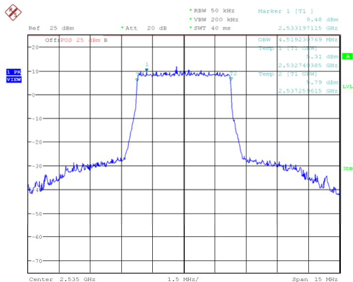
Fig.25 LTE band 7, 5MHz Bandwidth, QPSK (99% BW)
