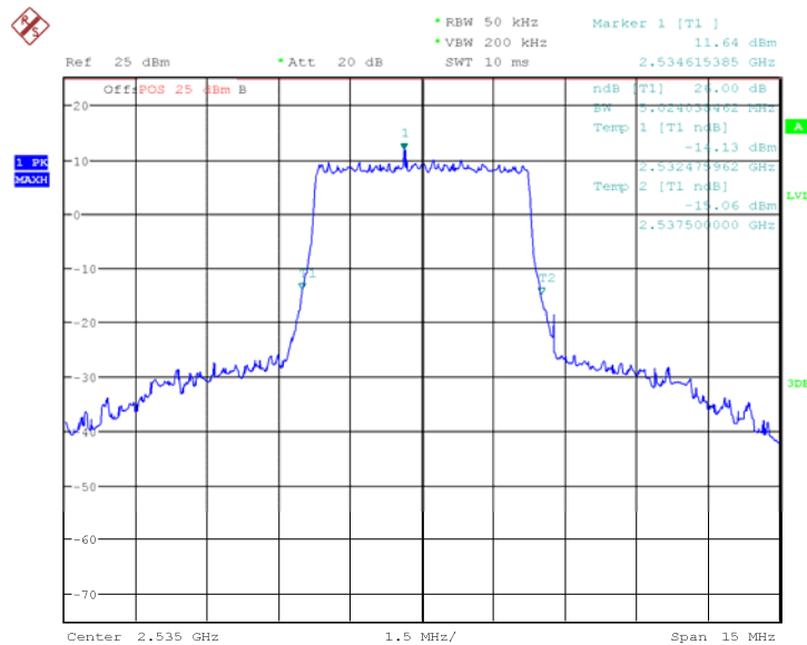
Fig.45 LTE band 7, 5MHz Bandwidth, QPSK (-26dBc BW)
