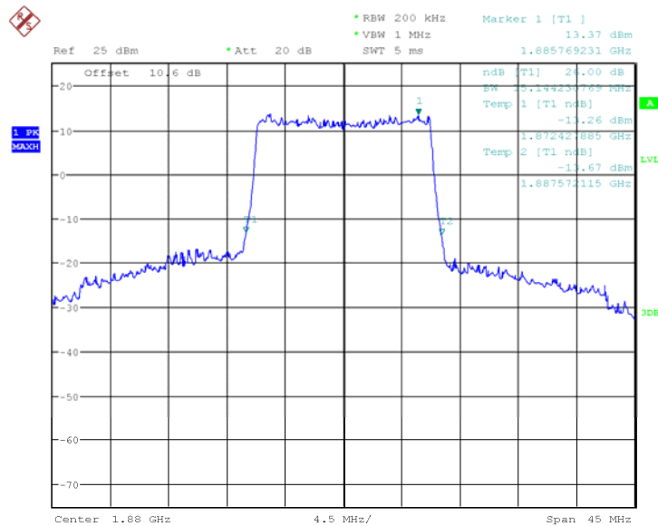
Fig.41 LTE band 2, 15MHz Bandwidth, QPSK (-26dBc BW)
