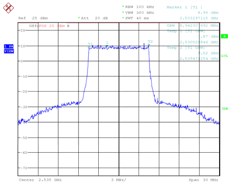
Fig.27 LTE band 7, 10MHz Bandwidth, QPSK (99% BW)
