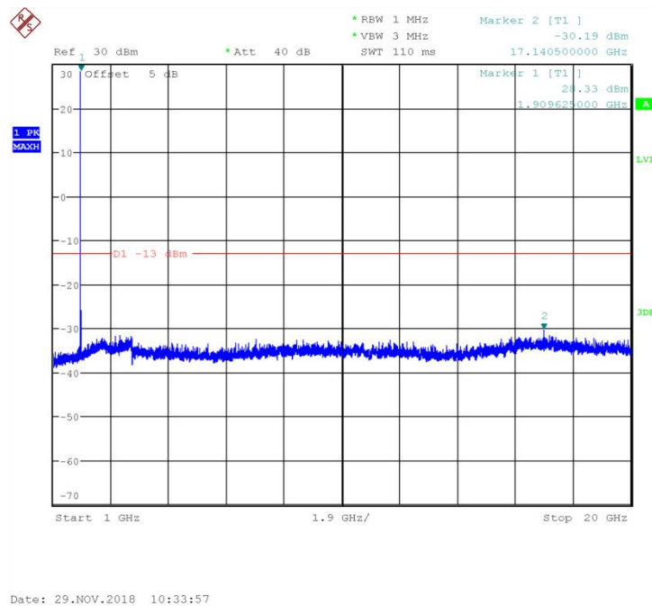
Fig.28 Channel 810: 1GHz~20GHz
