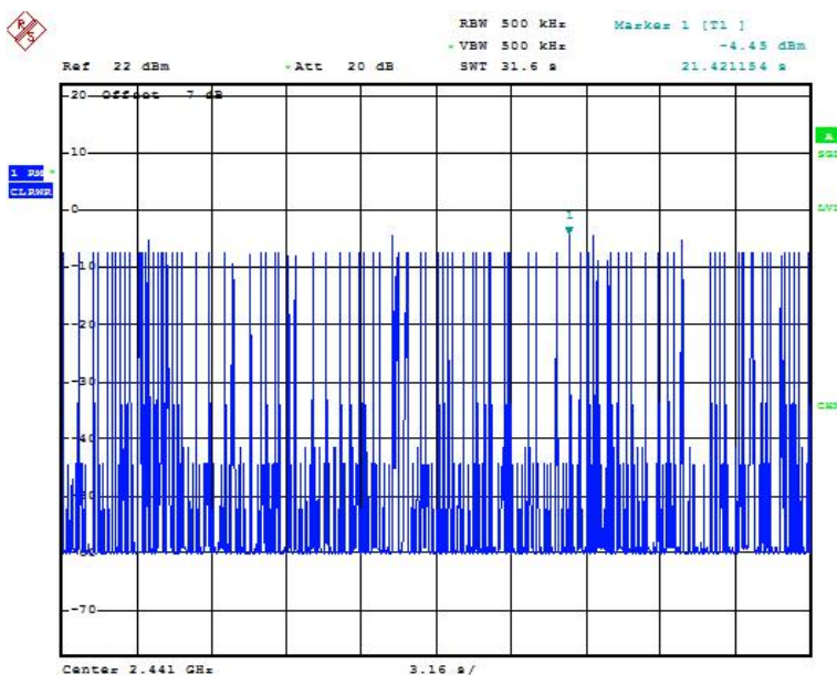
Fig.64 Time of occupancy (Dwell Time): Ch39,Packet DH5
