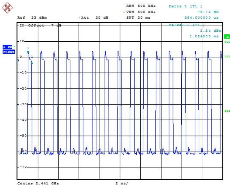
Fig.72 Time of occupancy (Dwell Time): Ch39,Packet 3-DH1
