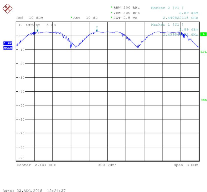
Fig.87 Carrier separation measurement: GFSK, Ch39
