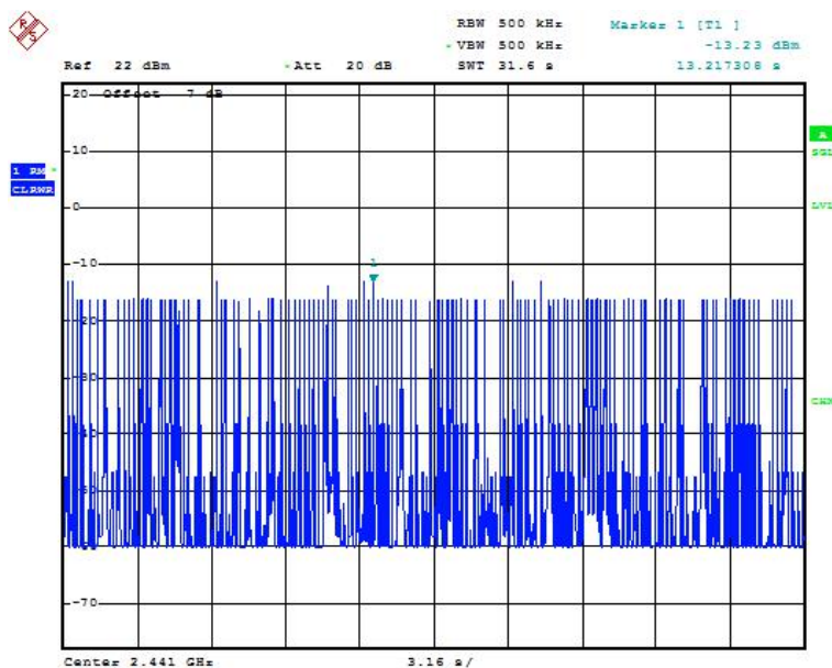
Fig.74 Time of occupancy (Dwell Time): Ch39,Packet 3-DH3
