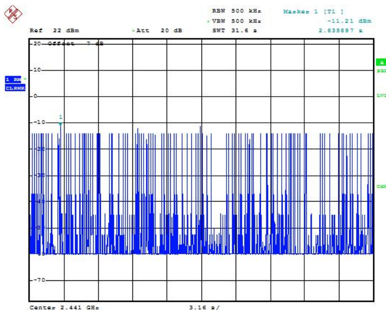
Fig.76 Time of occupancy (Dwell Time): Ch39,Packet 3-DH5
