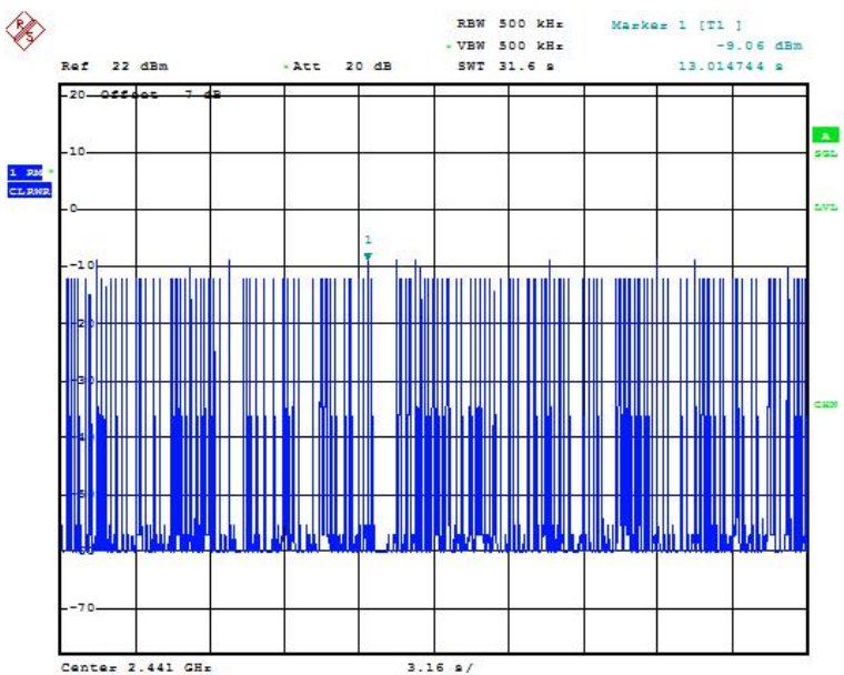
Fig.68 Time of occupancy (Dwell Time): Ch39,Packet 2-DH3
