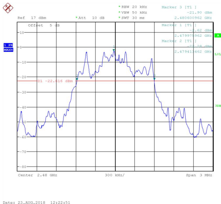
Fig.86 20dB Bandwidth: 8DPSK, Ch78
