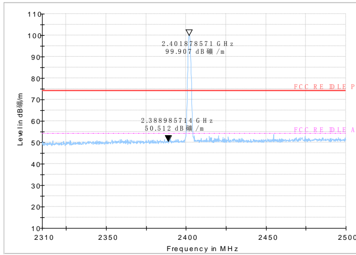
Fig.43 Radiated emission (Power): GFSK, low channel
