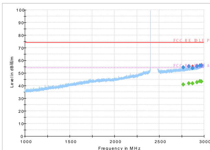
Fig.53 Radiated emission: 8DPSK, Ch0, 1GHz~3GHz
