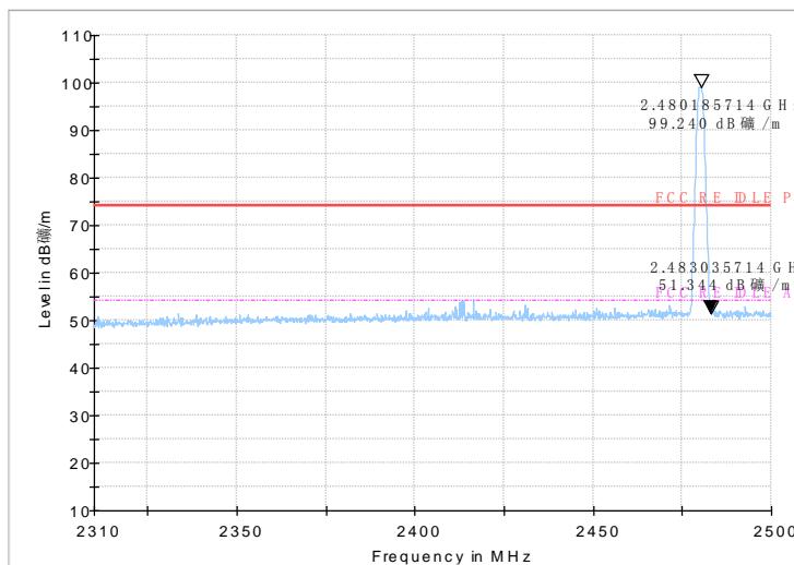
Fig.56 Radiated emission (Power): 8DPSK, high channel
