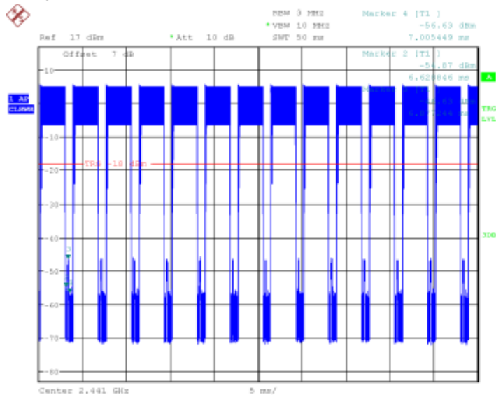
Fig.74 Time of occupancy (Dwell Time): Ch39,Packet 3-DH5
