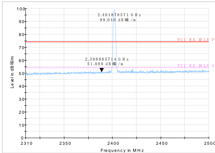
Fig.55 Radiated emission (Power): 8DPSK, low channel
