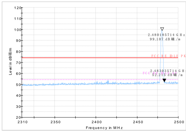
Fig.50 Radiated emission (Power): \pi/4 DQPSK, high channel
