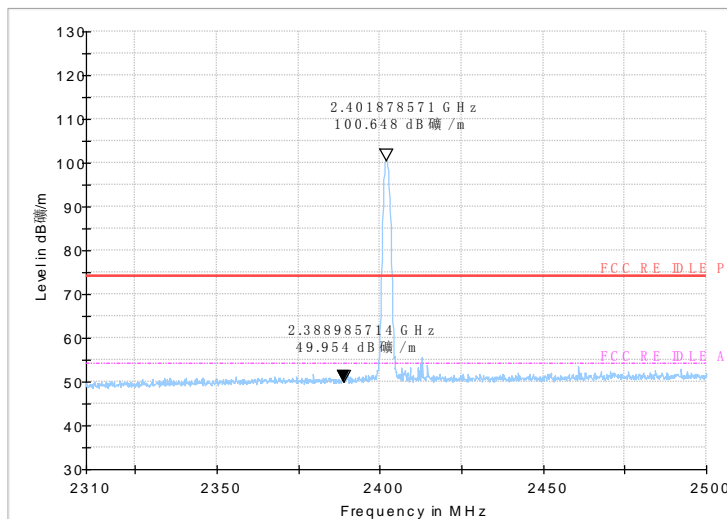
Fig.49 Radiated emission (Power): \pi/4 DQPSK, low channel
