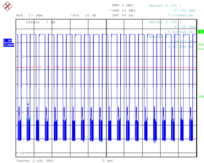
Fig.60 Time of occupancy (Dwell Time): Ch39, Packet DH3
