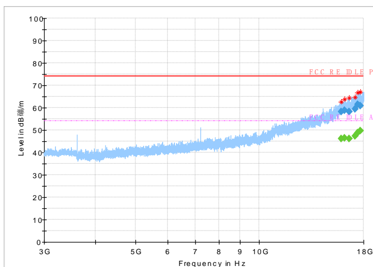
Fig.54 Radiated emission: 8DPSK, Ch0, 3GHz~18GHz
