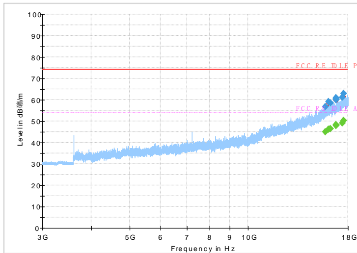
Fig.48 Radiated emission: \pi/4 DQPSK, Ch0, 3GHz~18GHz
