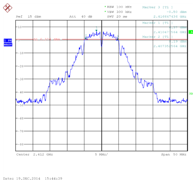
Fig.10 Occupied 6dB Bandwidth (802.11b, Ch1)
