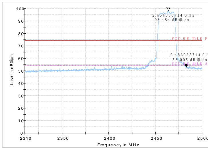
Fig.55 Radiated emission (Power): 802.11n, high channel
