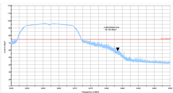
802.11g-Channel 11 Peak
