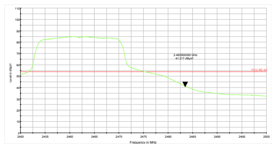
802.11g-Channel 11 Average
