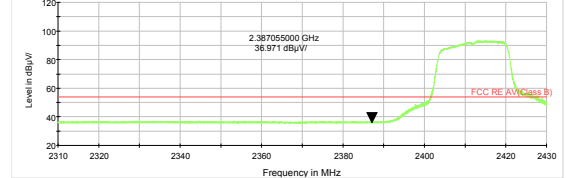
802.11g-Channel 1 Average
