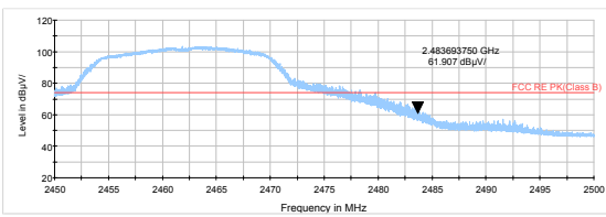
802.11g-Channel 11 Peak
