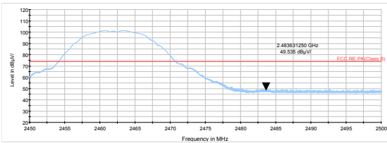
802.11b-Channel 11 Peak
