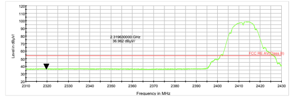
802.11b-Channel 1 Average
