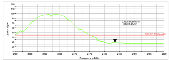
802.11b-Channel 11 Average
