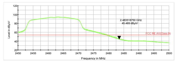
802.11g-Channel 11 Average
