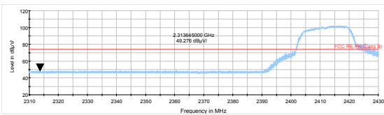
802.11g-Channel 1 Peak
