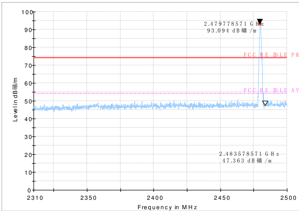
Peak detector
