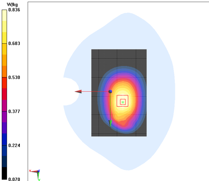
Fig.3 GSM 850MHz Ground Mode High Repeated
