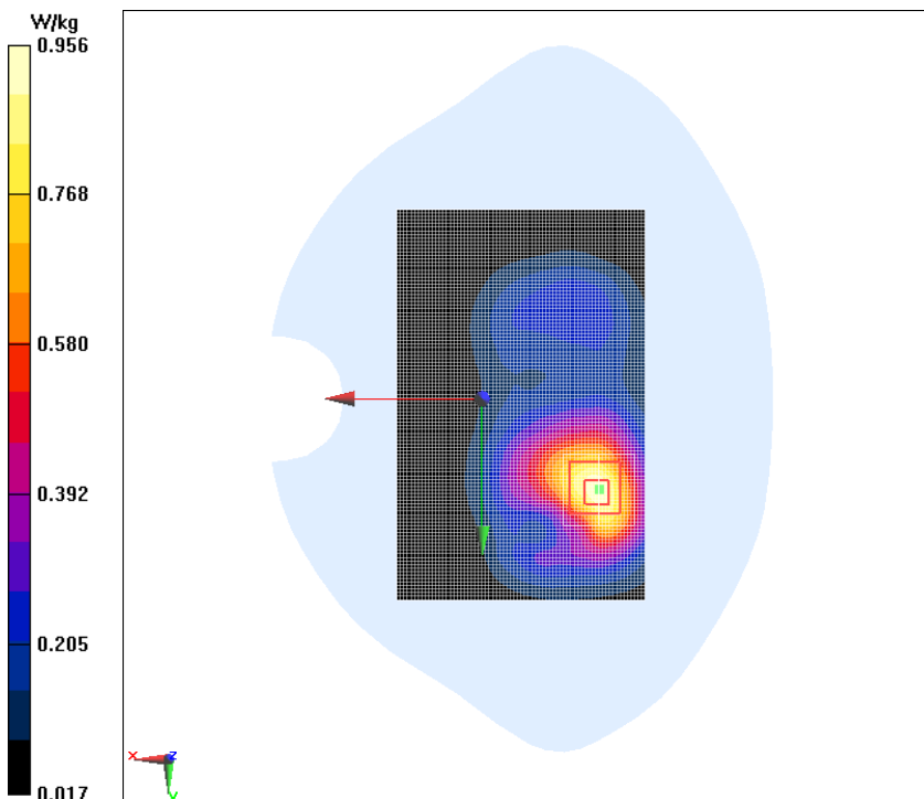
Fig.6 GSM 1900MHz Ground Mode High
