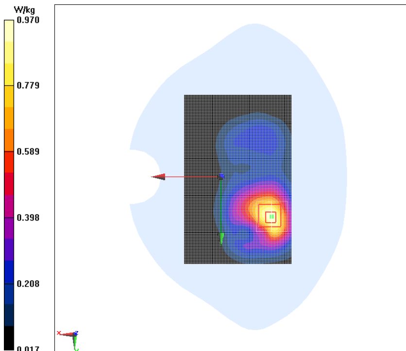
Fig.7 GSM 1900MHz Ground Mode High Repeated
