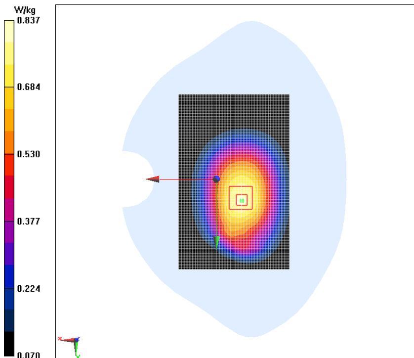
Fig.2 GSM 850MHz Ground Mode High
