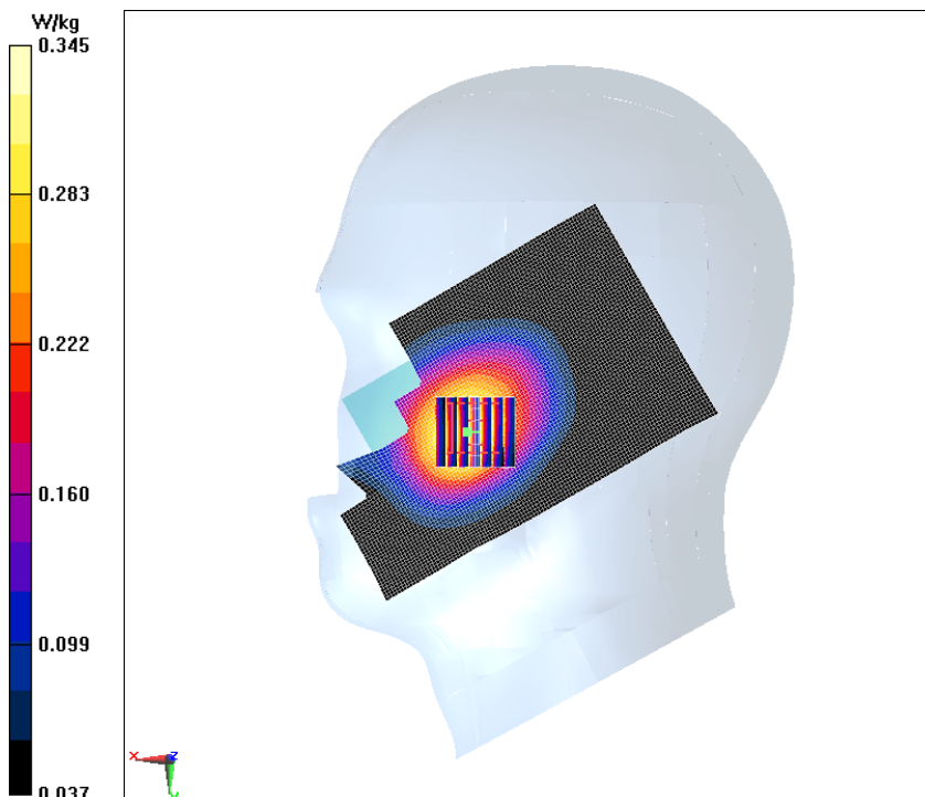
Fig.1 GSM 850MHz Right Cheek High
