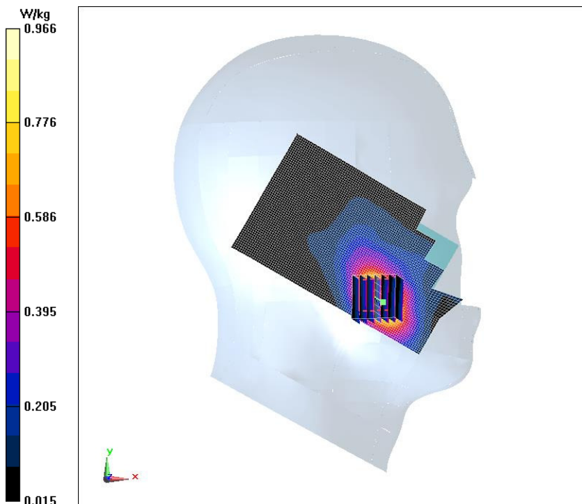
Fig.5 GSM 1900MHz Left Cheek Low Repeated
