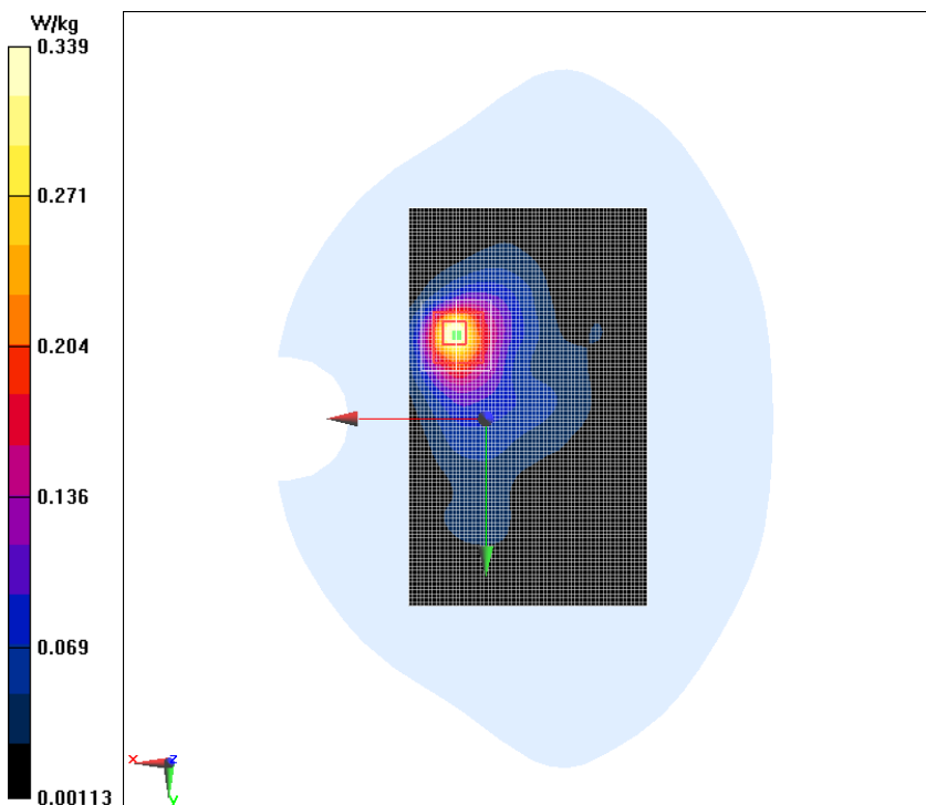
Fig.9 WiFi 802.11b Phantom Mode Middle
