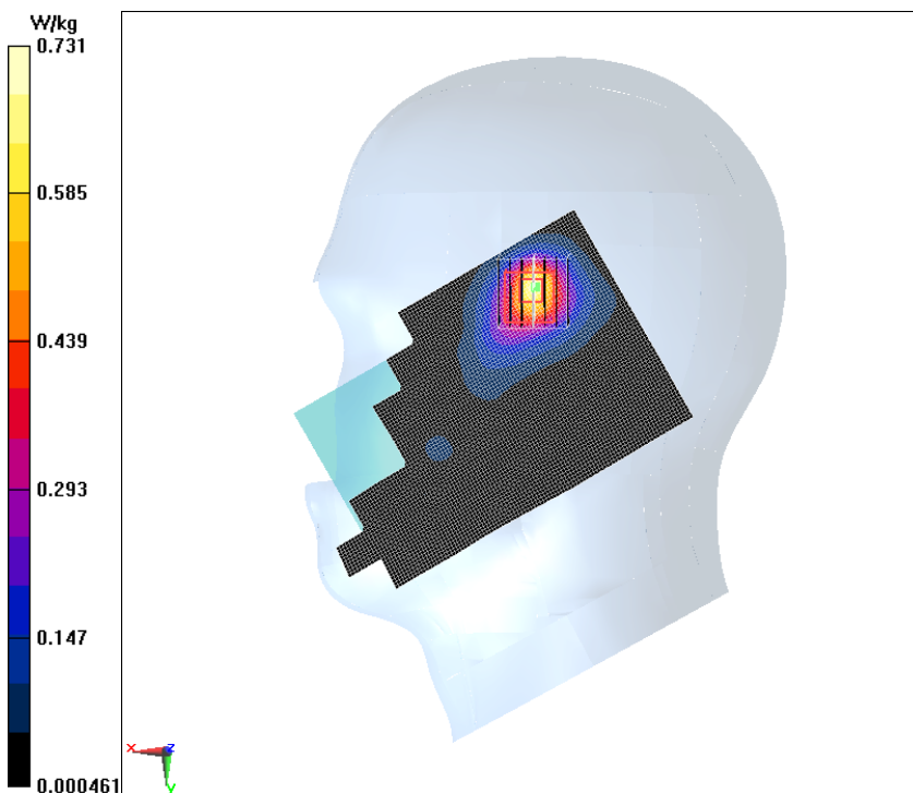
Fig.8 WiFi 802.11b Right Cheek Low
