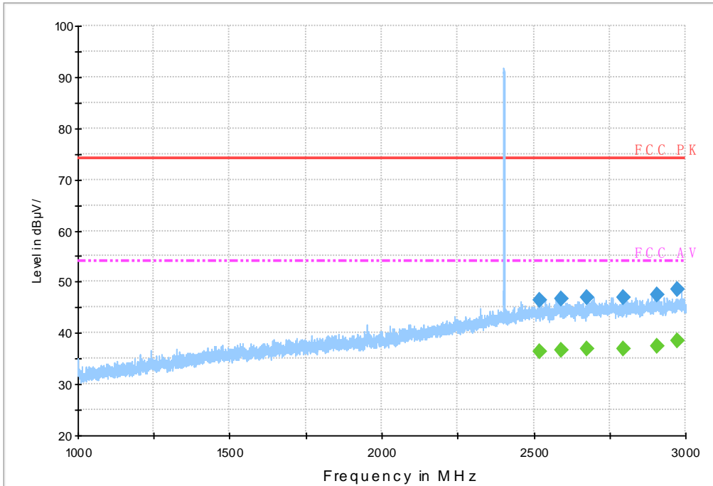
Fig.46 Radiated emission: \pi/4 DQPSK, Ch0, 1GHz~3GHz
