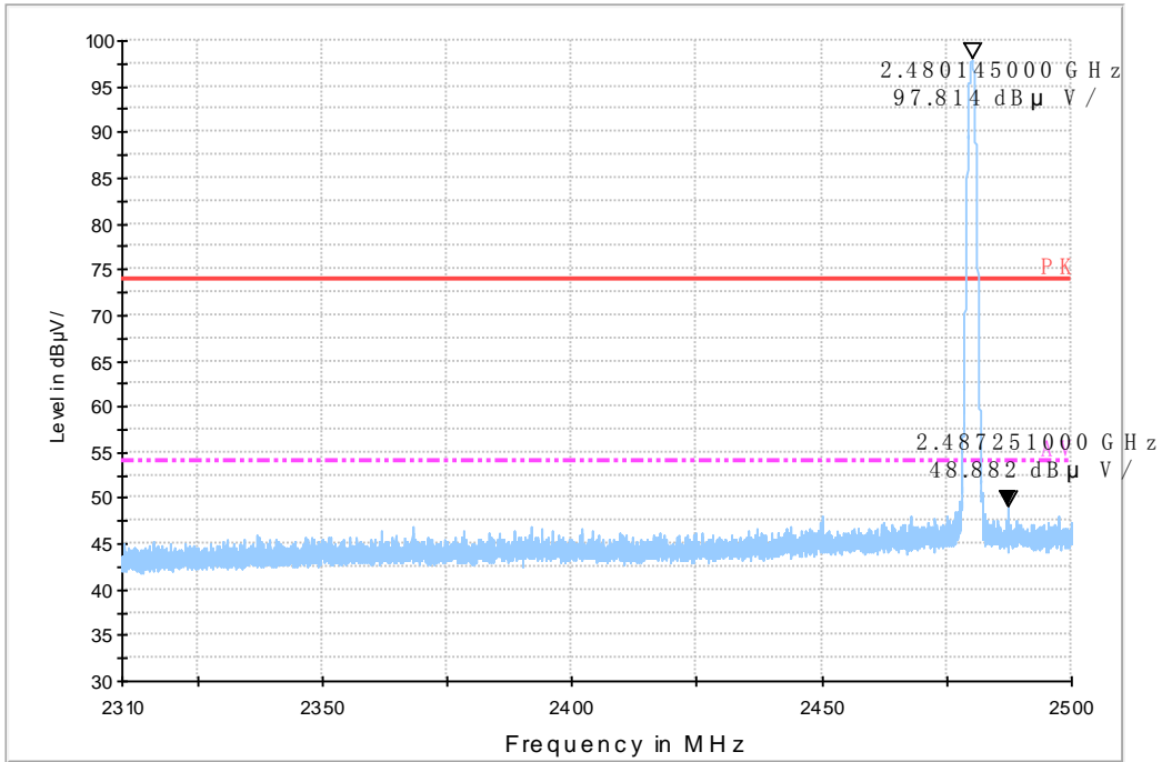
Fig.44 Radiated emission (Power): GFSK, high channel
