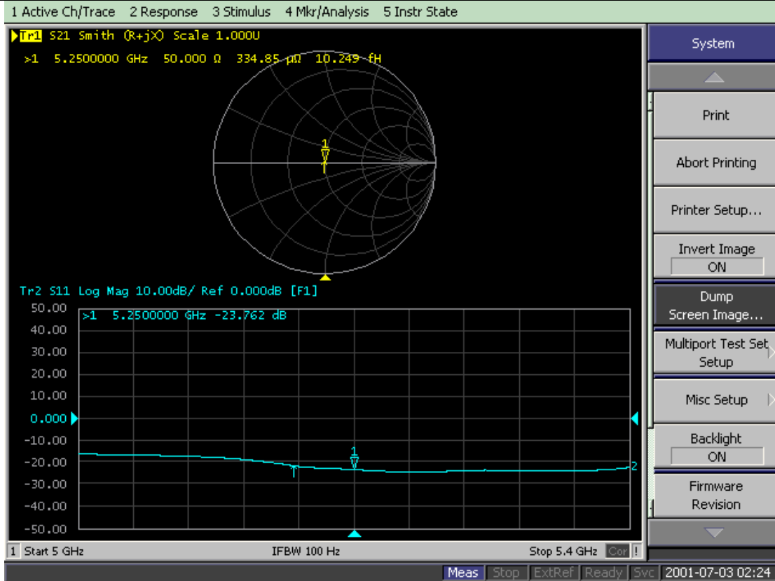
D5GHzV2-5250MHz-Head-1/4/2018
