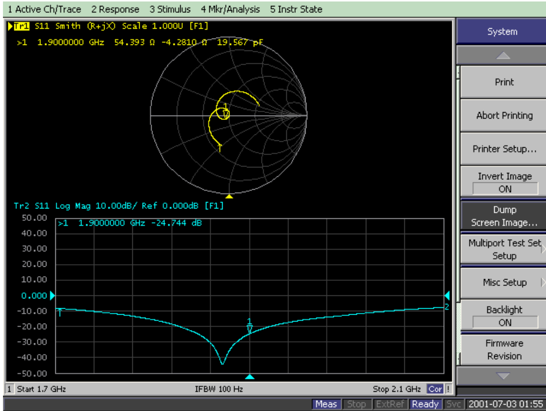
D1900V2-Head-8/25/2018
