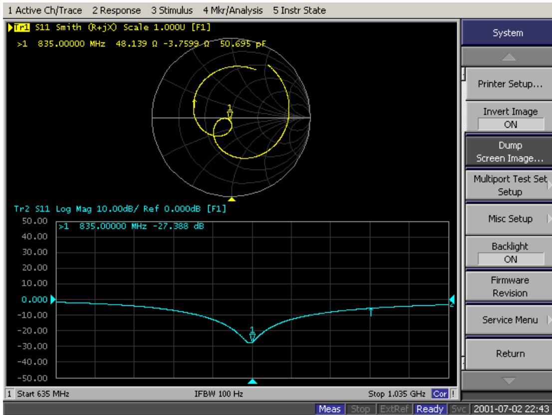
D835V2-Body-8/27/2018
