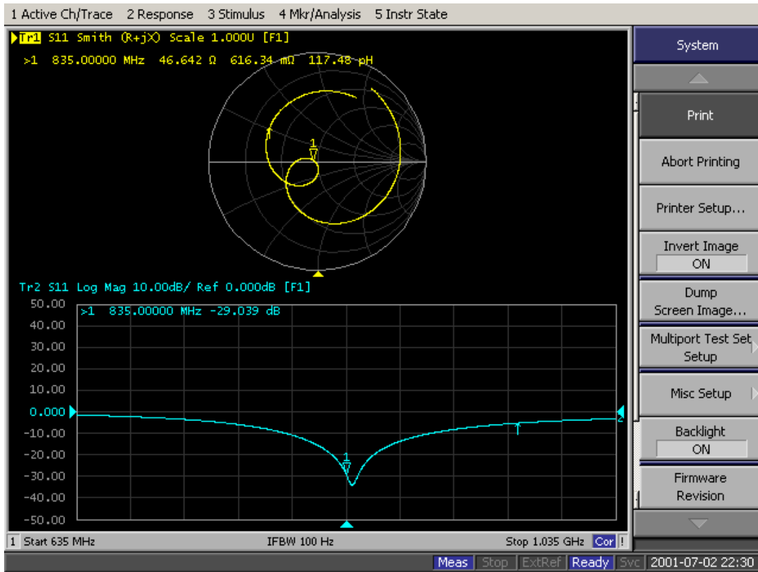
D835V2-Head-8/27/2018
