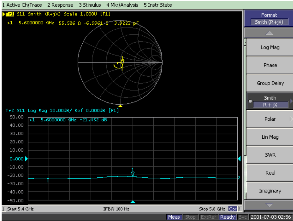
D5GHzV2-5600MHz-Head-1/4/2018
