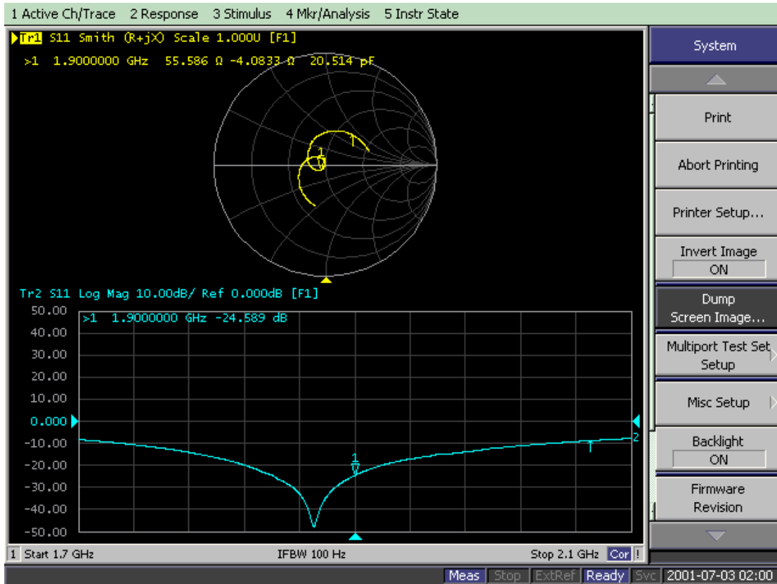
D1900V2-Body-8/25/2018
