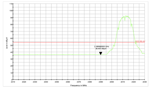
802.11b-Channel 1 Average
