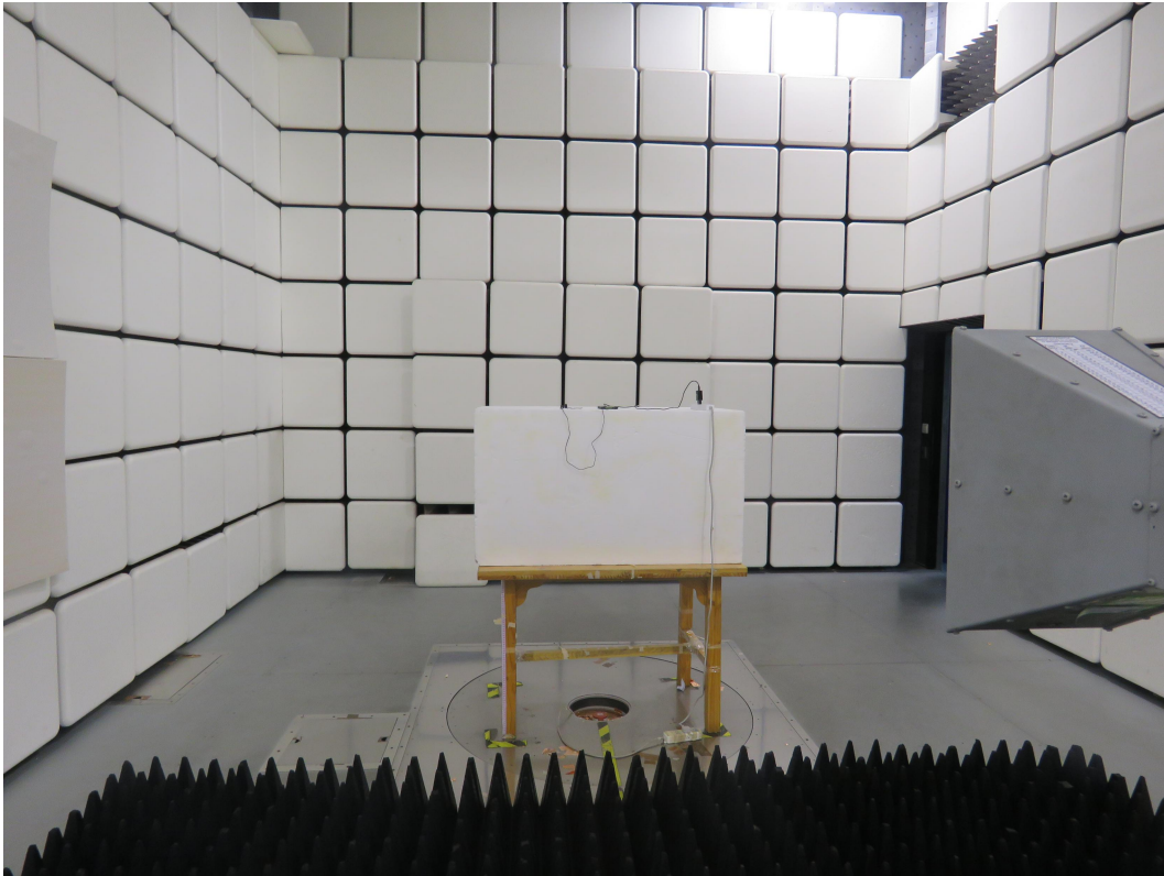
Above 1GHz Picture 2 Radiated Emission Test Setup
