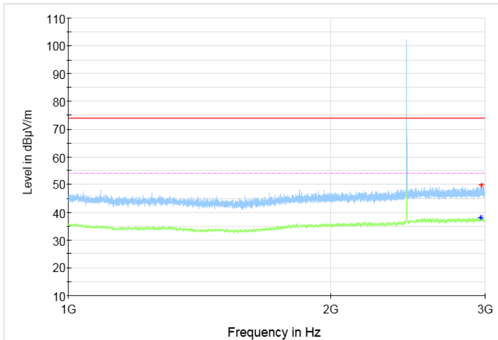
Fig.22 Radiated Spurious Emission (GFSK, Ch19, 1 GHz ~3 GHz)
