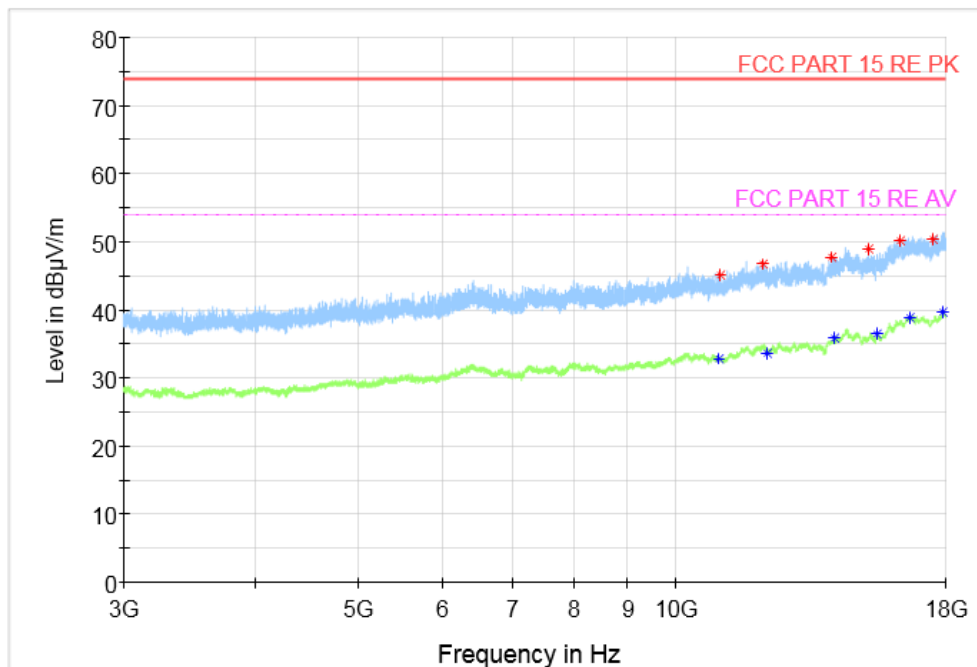
Fig.21 Radiated Spurious Emission (GFSK, Ch0, 3 GHz ~18 GHz)
