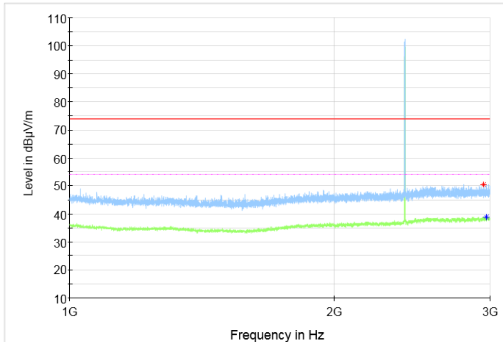
Fig.20 Radiated Spurious Emission (GFSK, Ch0, 1 GHz ~3 GHz)
