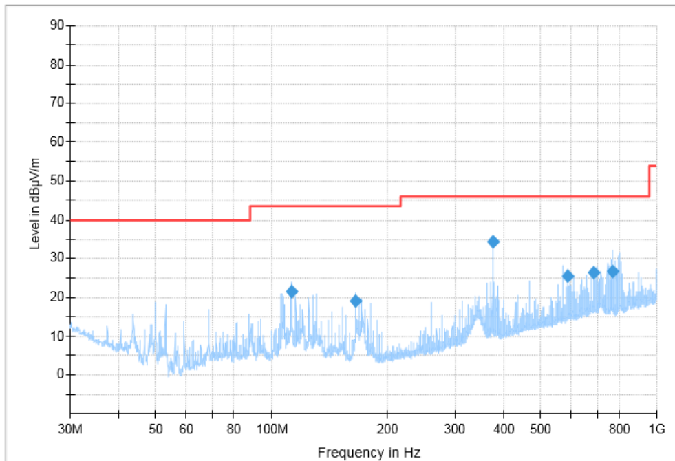
Fig.29 Radiated Spurious Emission (All Channels, 30 MHz-1 GHz)
