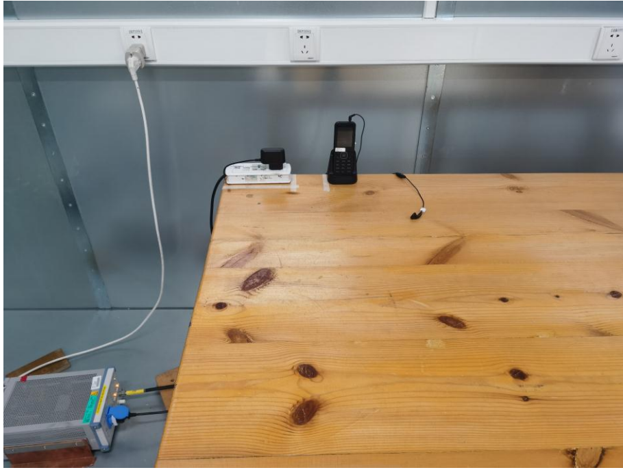
11. Conducted Emission (Part 15B, Charging mode with Charging cradle)
