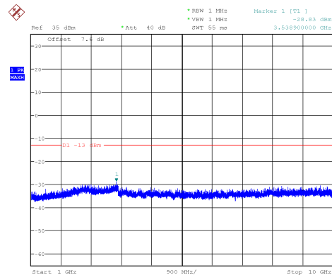
Channel 251: 1GHz~10GHz
