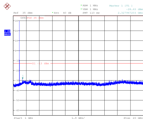
Channel 661: 1GHz~20GHz
