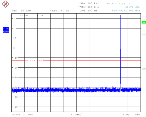
Channel 251: 30MHz~1GHz
