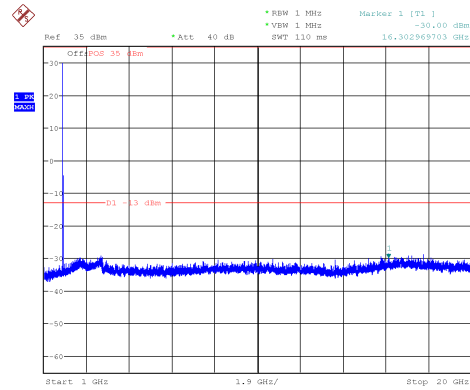
Channel 512: 1GHz~20GHz
