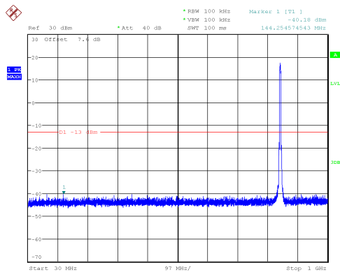
Channel 4232: 30MHz~1GHz
