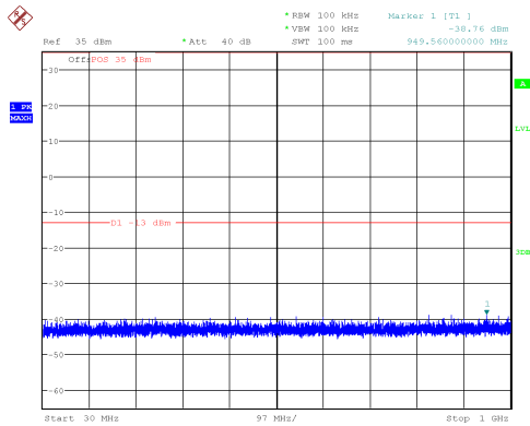
Channel 661: 30MHz~1GHz
