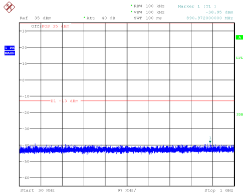
Channel 512: 30MHz~1GHz
