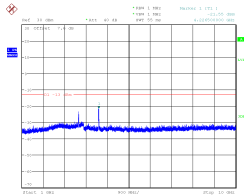
Channel 4232: 1GHz~10GHz
