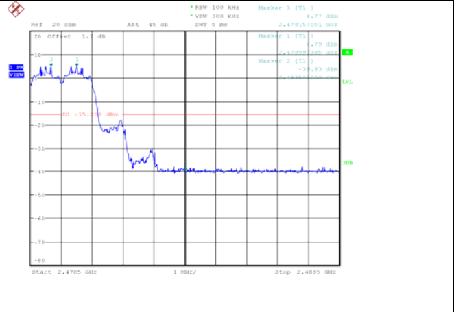
Frequency Band Edge: 8DPSK, Ch78, Hopping ON
