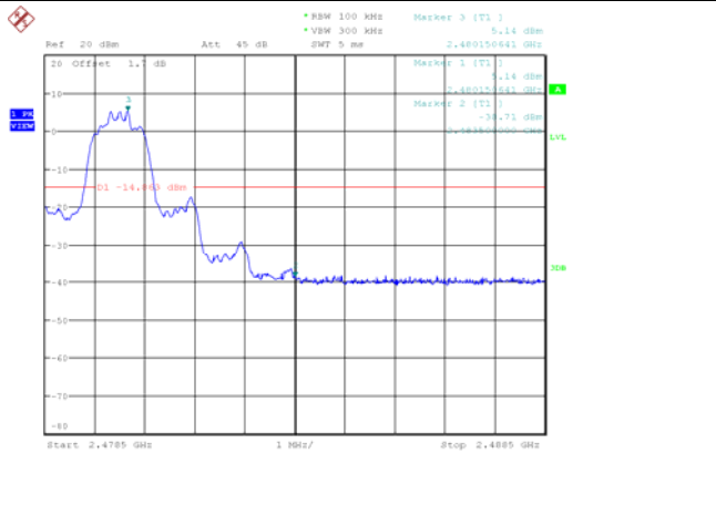
Frequency Band Edge:8DPSK,Ch78, Hopping OFF
