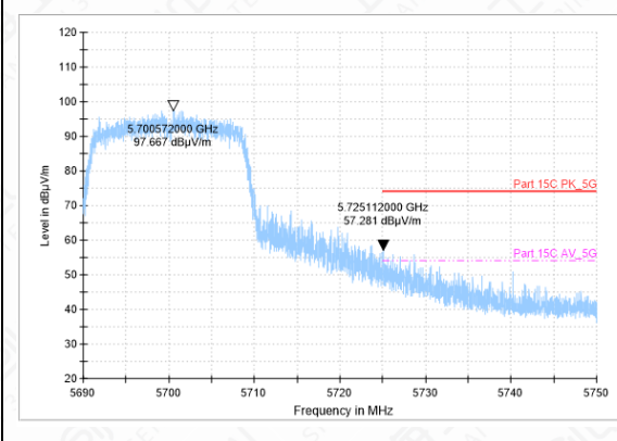
Peak detector
