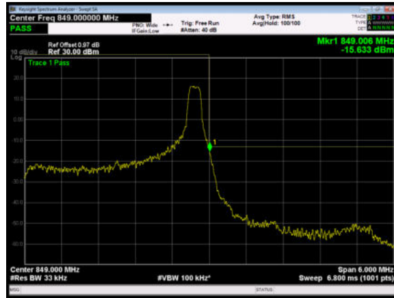
LTE Band 5 QPSK 3MHz CH-High 100%RB
