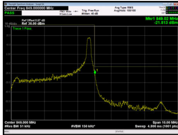
LTE Band 5 QPSK 5MHz CH-High 1RB
