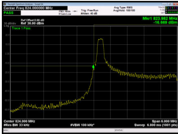
LTE Band 5 QPSK 3MHz CH-Low 100%RB
