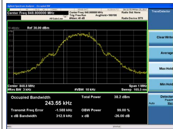
GSM 850 CH-High
