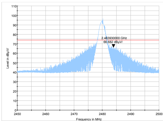
DH5-Channel 78: Peak
